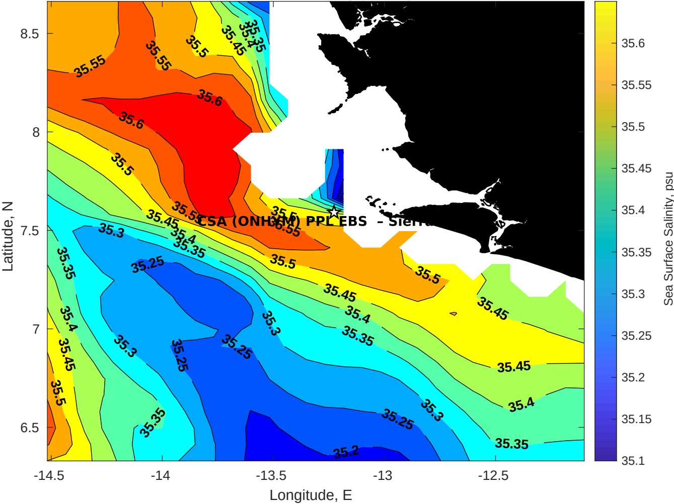
Surface Salinity for CSA (ONHYM) PPL EBS - Sierra Leone at 05-May-2025 00:00:00
