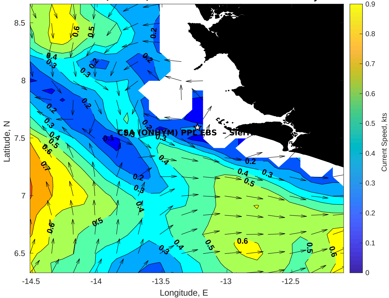
Surface Currents for CSA (ONHYM) PPL EBS - Sierra Leone at 05-May-2025 00:00:00
