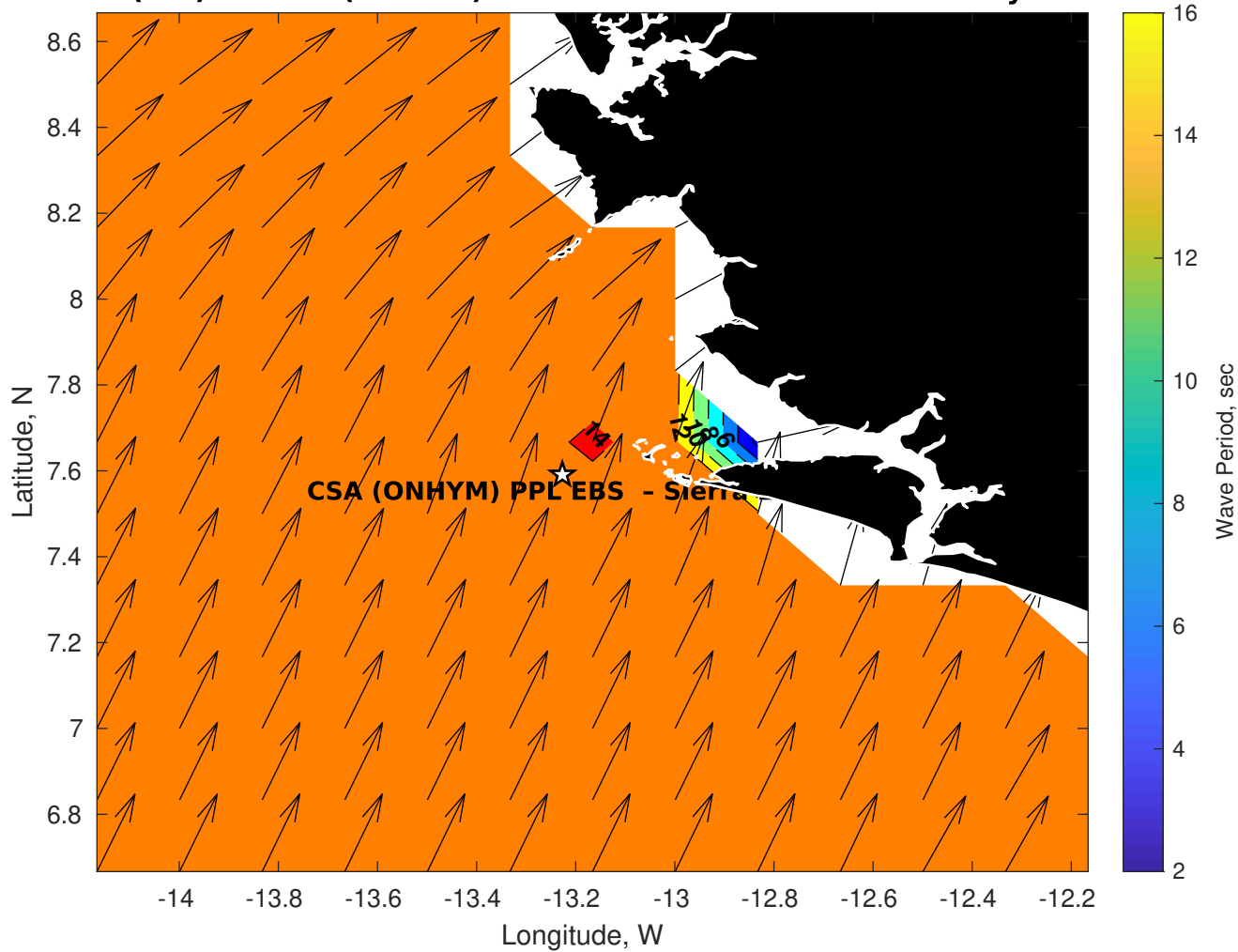
Wave Period (sec) for CSA (ONHYM) PPL EBS - Sierra Leone at 06-May-2025 09:00:00
