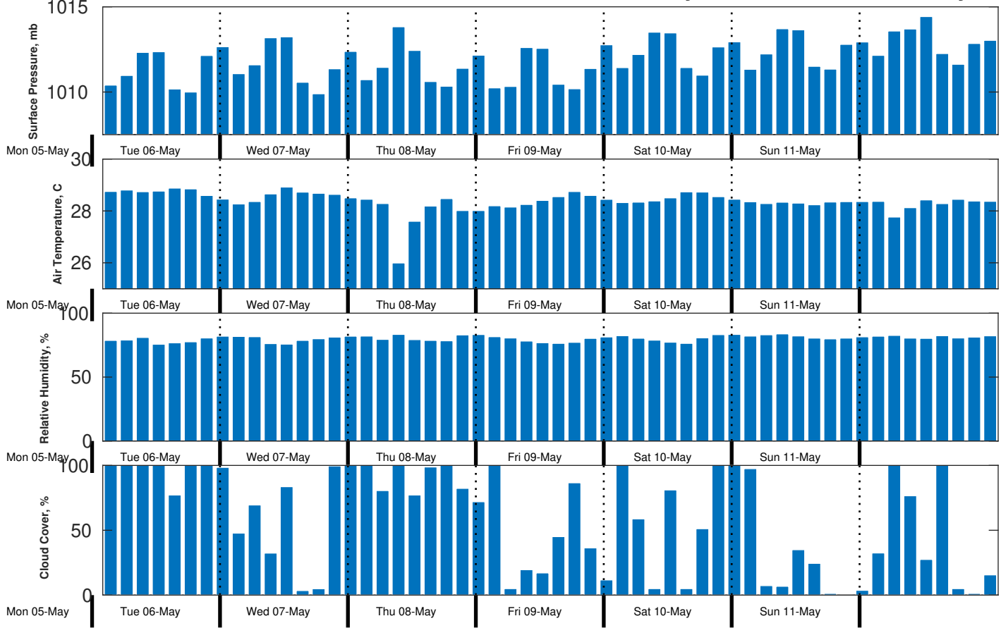
Met Forecast for CSA (ONHYM) PPL EBS - Sierra Leone from 06-May-2025 00:00:00 to 13-May-2025 00:00:00
