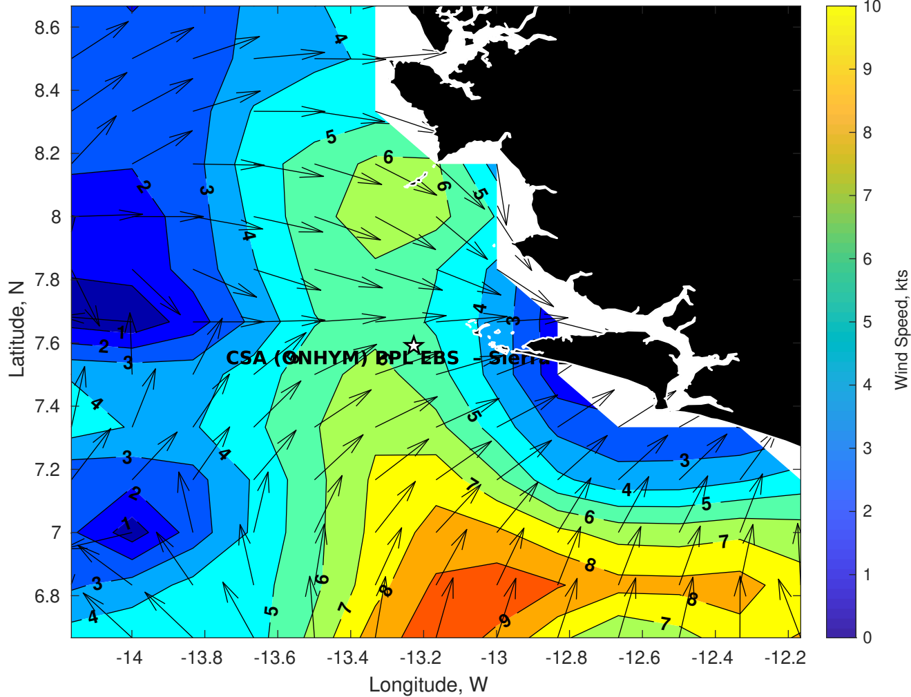
Winds (kts) for CSA (ONHYM) PPL EBS - Sierra Leone at 06-May-2025 09:00:00
