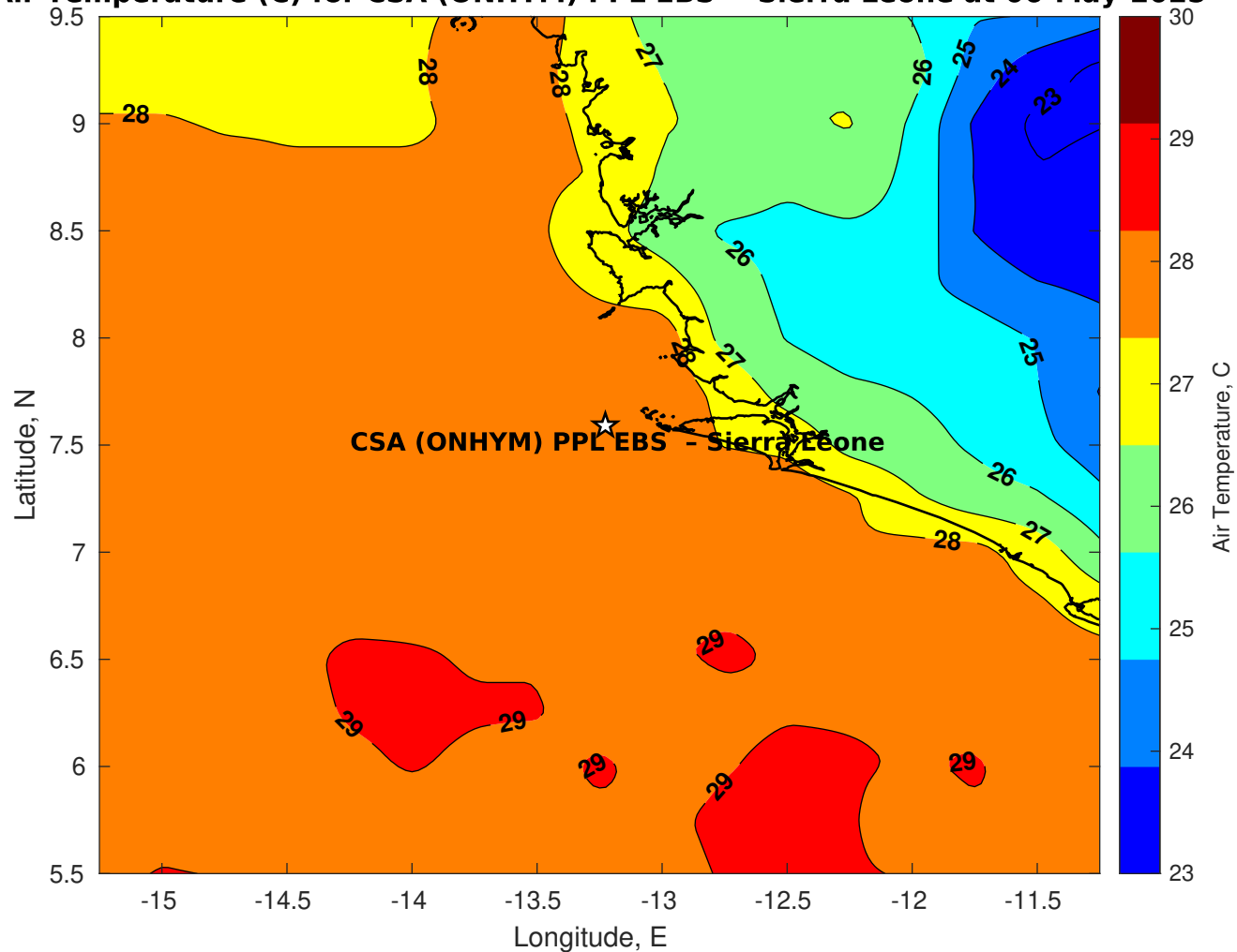
Air Temperature (C) for CSA (ONHYM) PPL EBS - Sierra Leone at 06-May-2025
