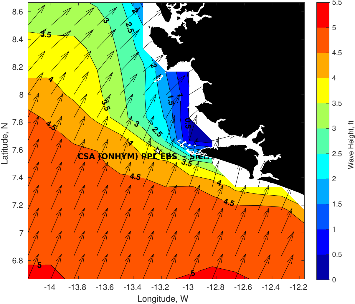
Wave Height (ft) for CSA (ONHYM) PPL EBS - Sierra Leone at 06-May-2025 09:00:00
