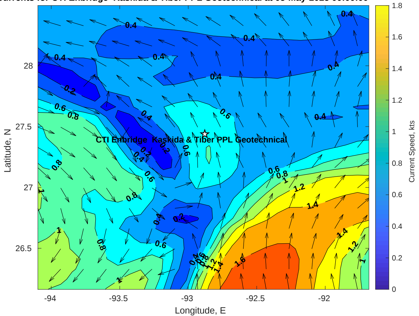
Surface Currents for CTI Enbridge Kaskida & Tiber PPL Geotechnical at 05-May-2025 00:00:00
