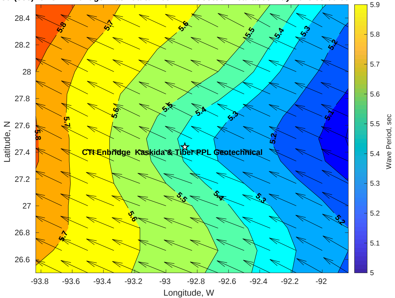
Wave Period (sec) for CTI Enbridge Kaskida & Tiber PPL Geotechnical at 06-May-2025 09:00:00
