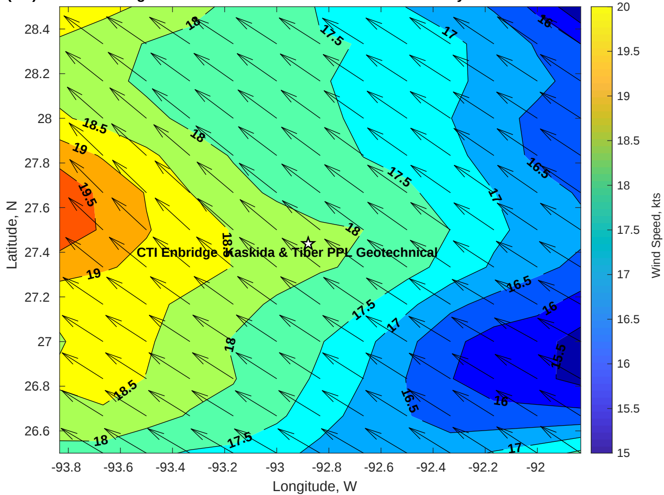
Winds (kts) for CTI Enbridge Kaskida & Tiber PPL Geotechnical at 06-May-2025 09:00:00
