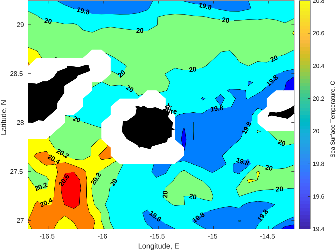
SST for Gyre at 05-May-2025 00:00:00
