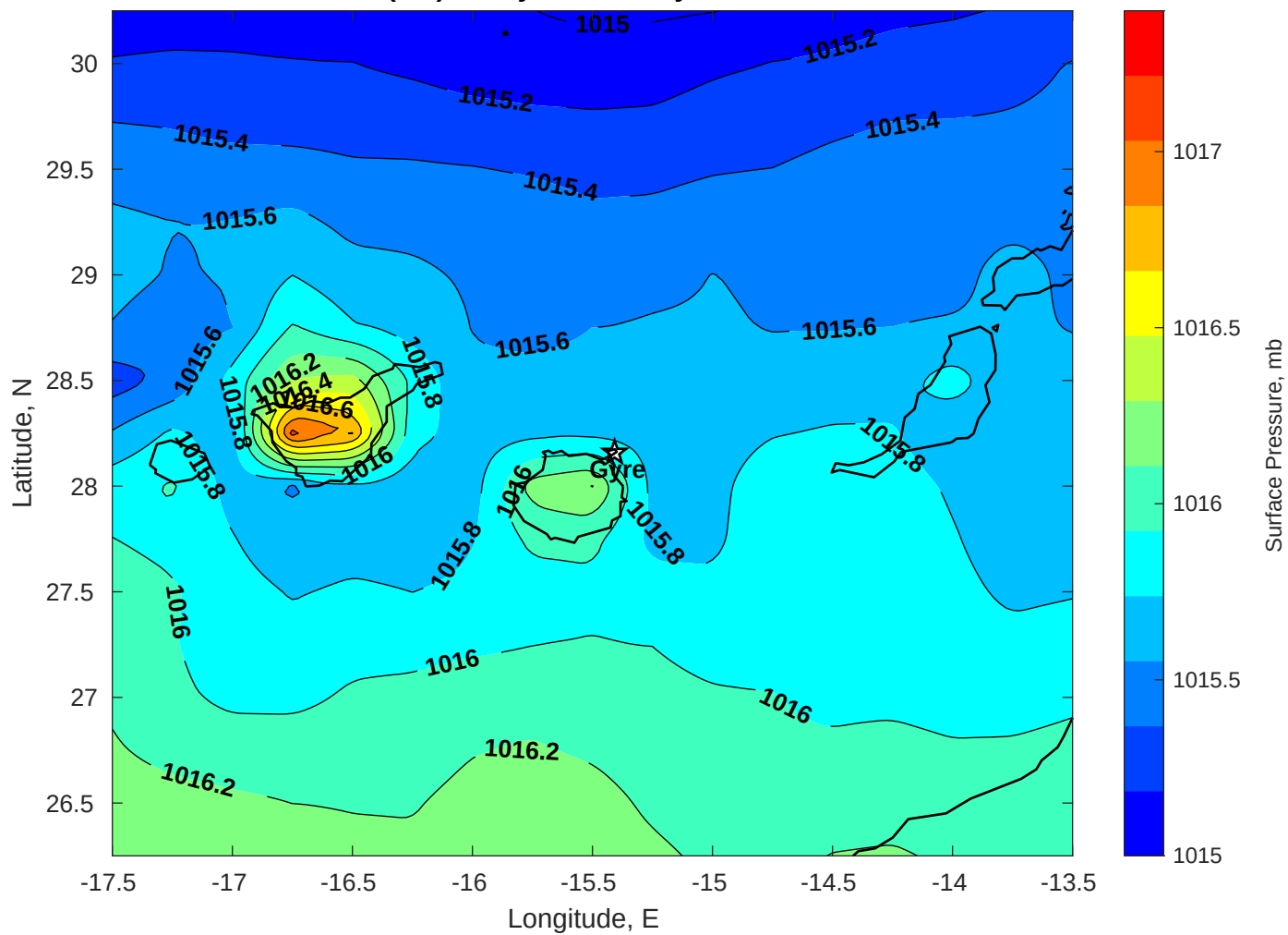
Surface Pressure (mb) for Gyre at 08-May-2025 00:00:00
