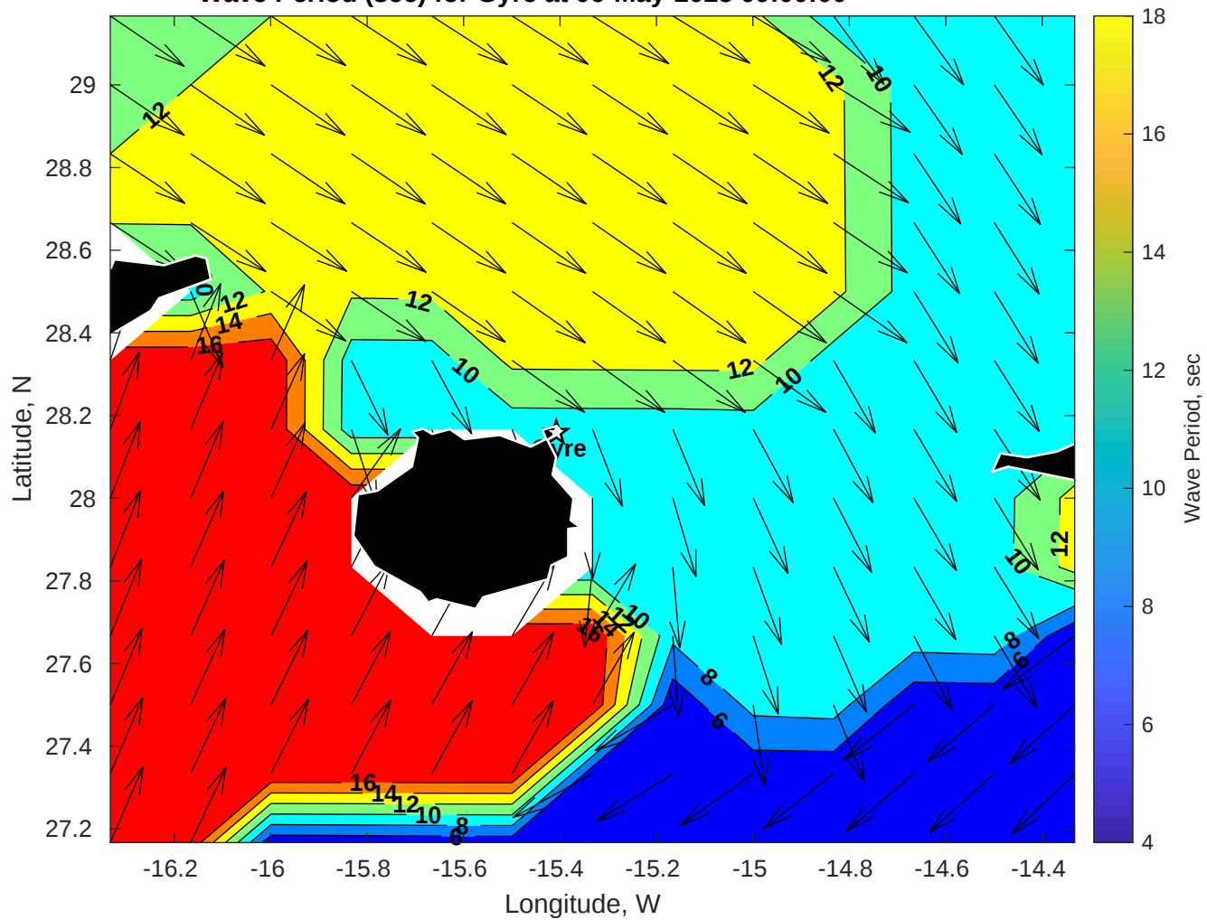
Wave Period (sec) for Gyre at 06-May-2025 09:00:00
