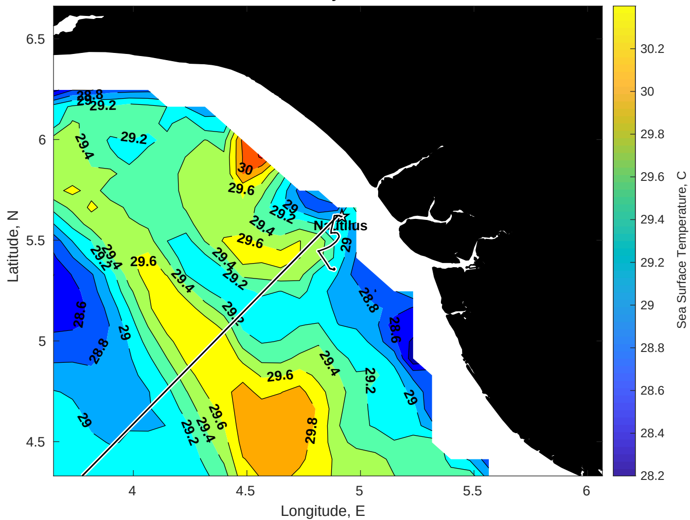
SST for Nautilus at 05-May-2025 00:00:00
