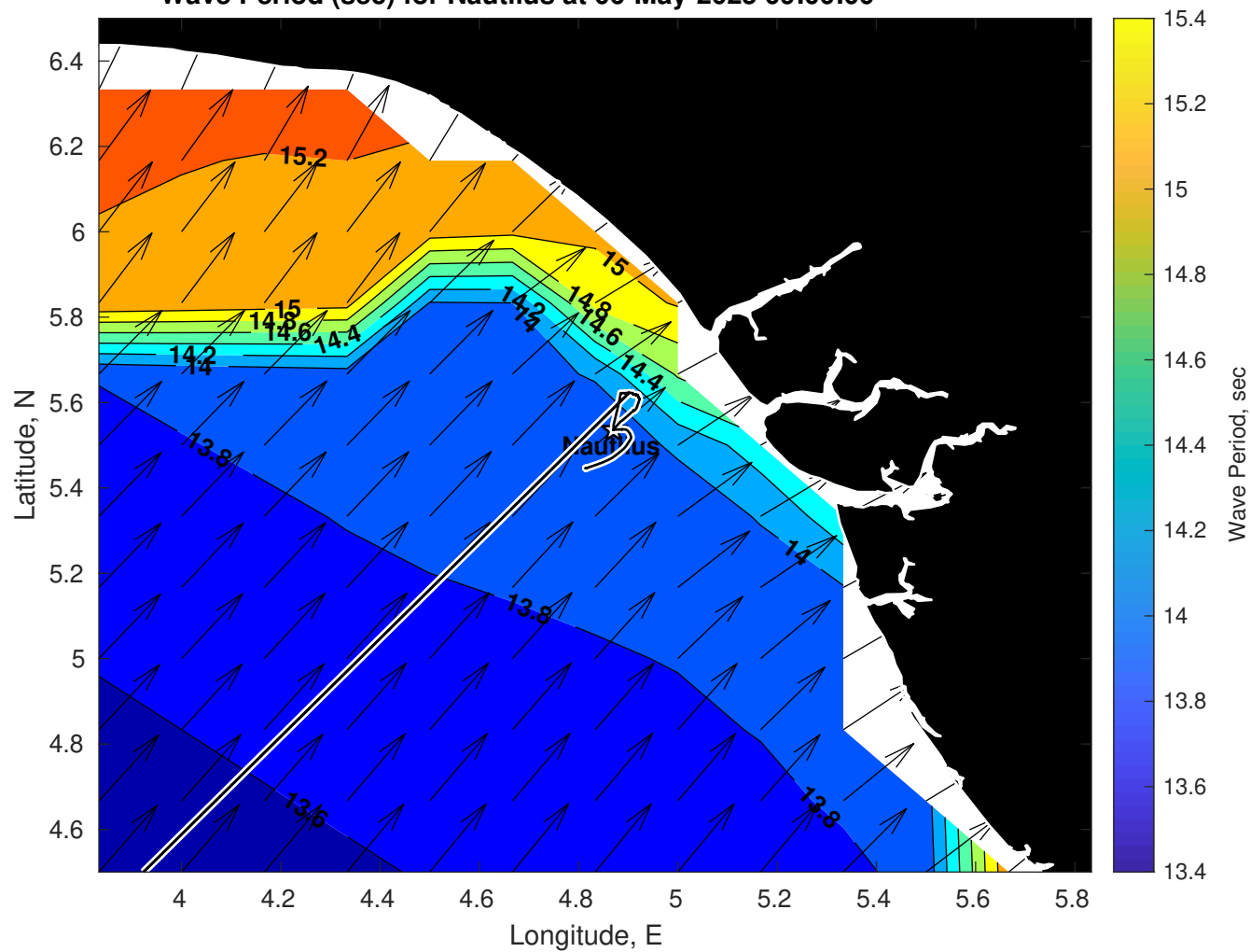
Wave Period (sec) for Nautilus at 06-May-2025 09:00:00
