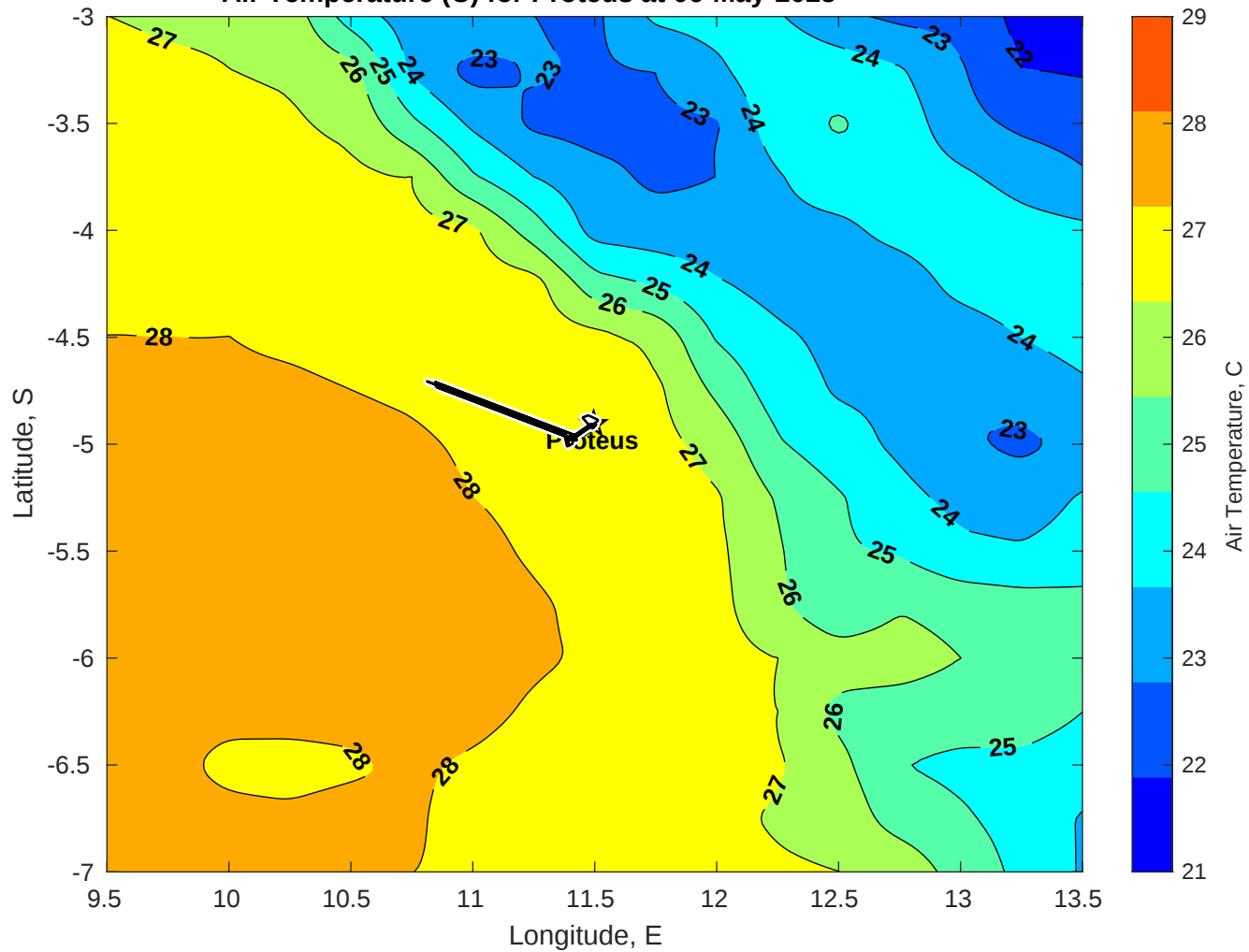
Air Temperature (C) for Proteus at 06-May-2025
