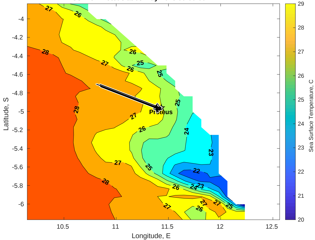
SST for Proteus at 05-May-2025 00:00:00
