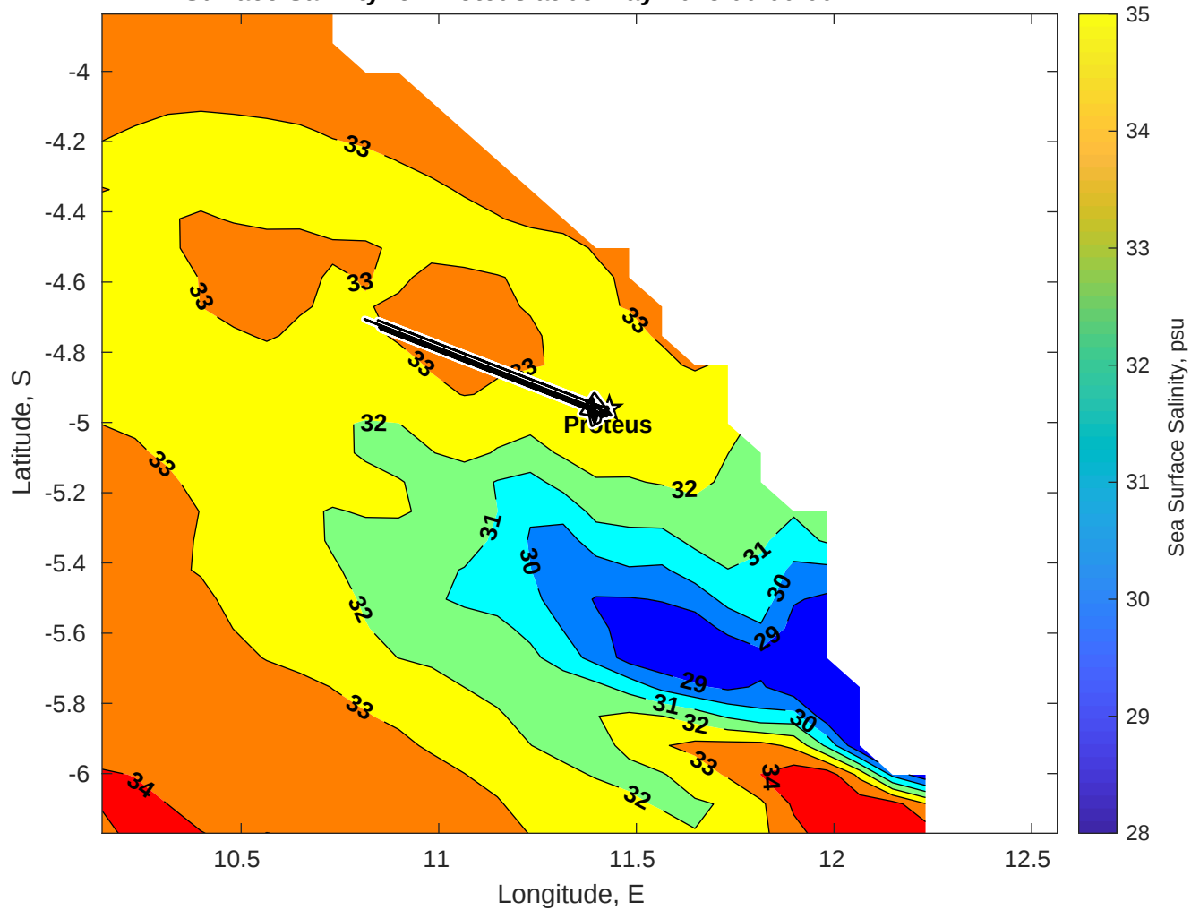
Surface Salinity for Proteus at 05-May-2025 00:00:00
