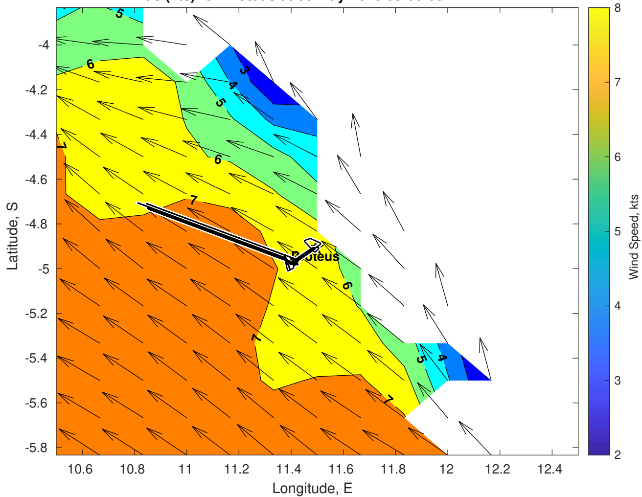
Winds (kts) for Proteus at 06-May-2025 09:00:00
