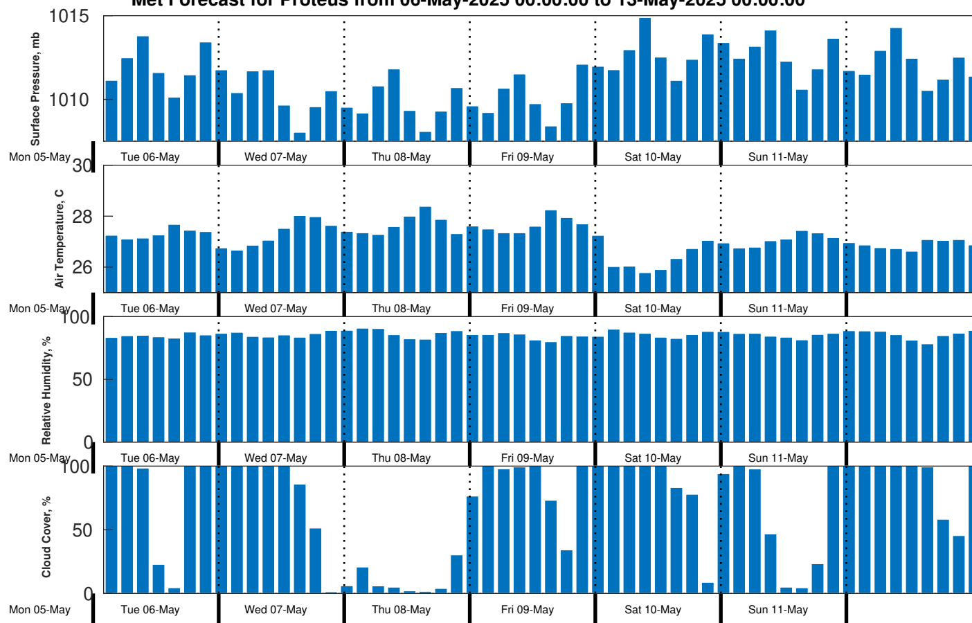
Met Forecast for Proteus from 06-May-2025 00:00:00 to 13-May-2025 00:00:00
