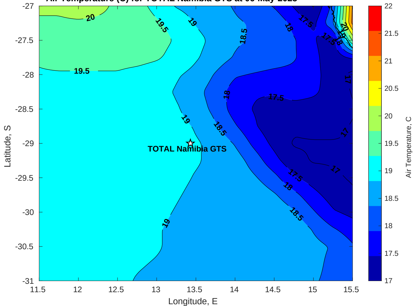
Air Temperature (C) for TOTAL Namibia GTS at 06-May-2025
