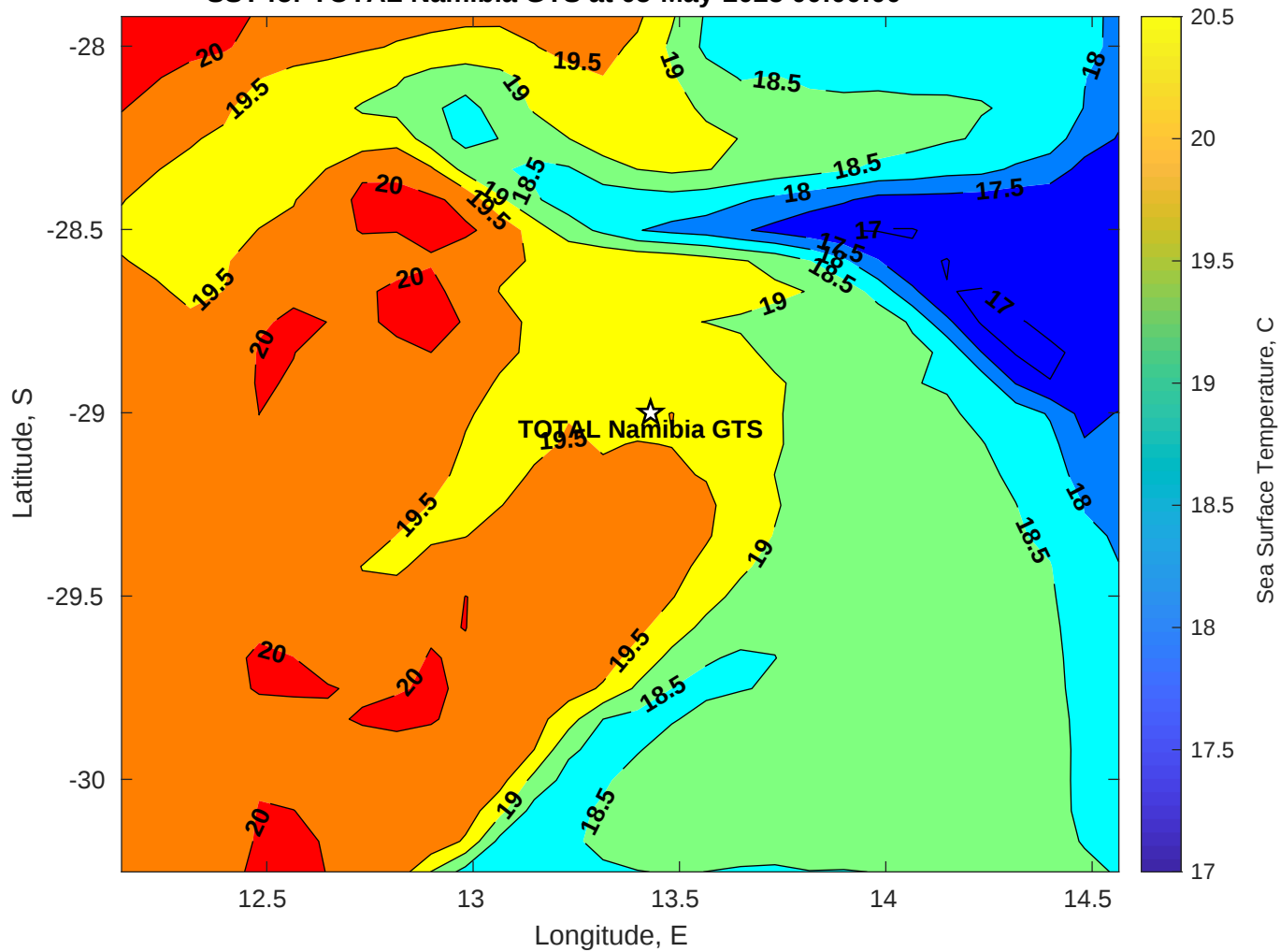
SST for TOTAL Namibia GTS at 05-May-2025 00:00:00
