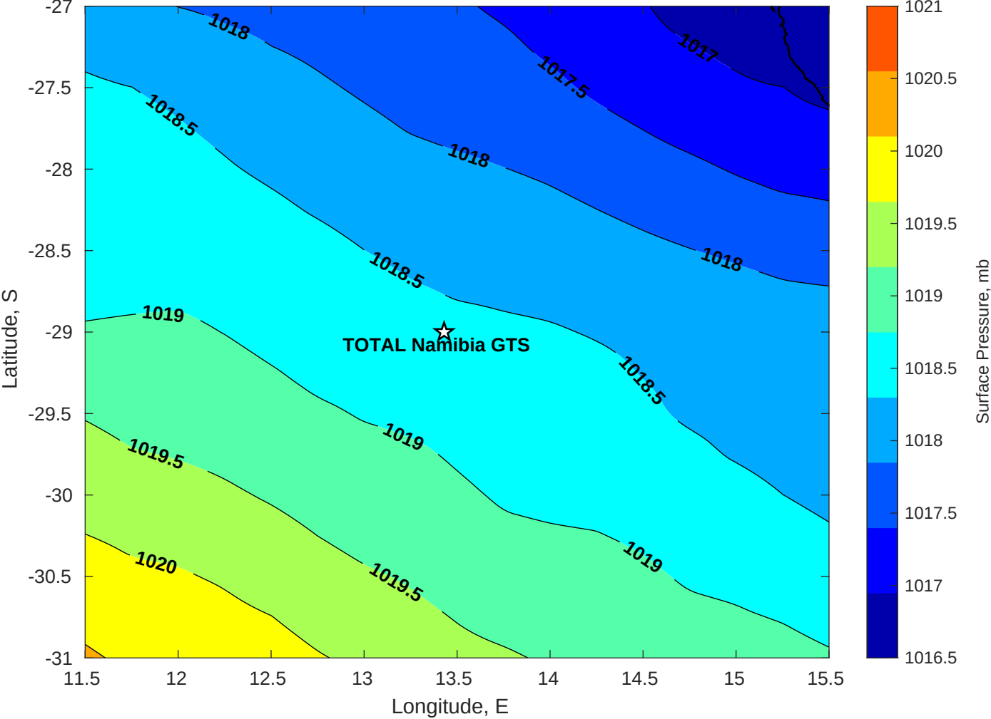
Surface Pressure (mb) for TOTAL Namibia GTS at 07-May-2025 00:00:00
