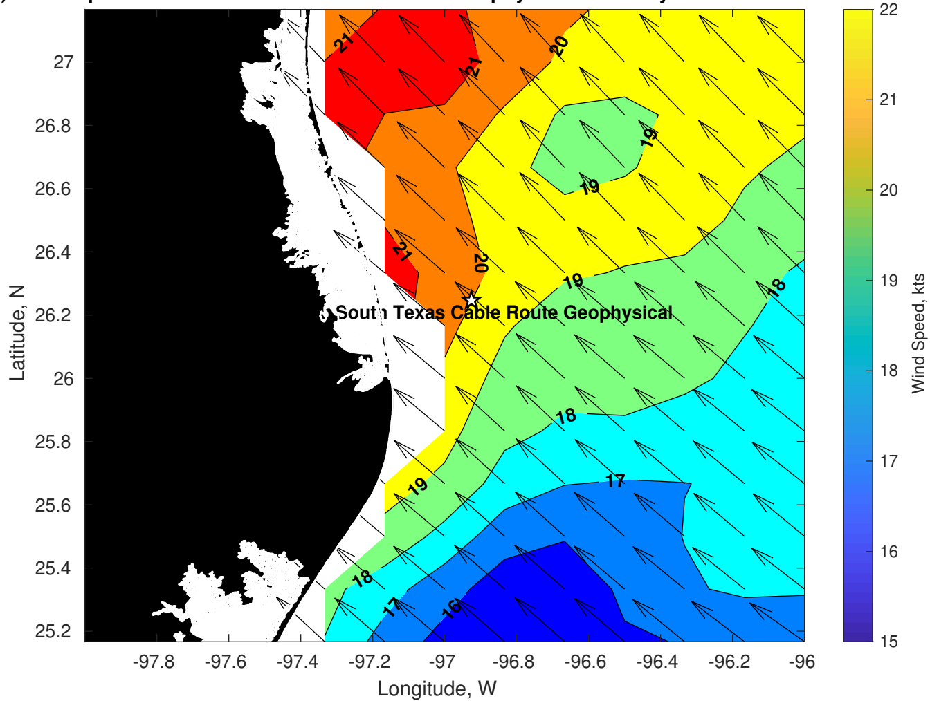
Winds (kts) for Tampnet P2378 South Texas Cable Route Geophysical at 06-May-2025 09:00:00
