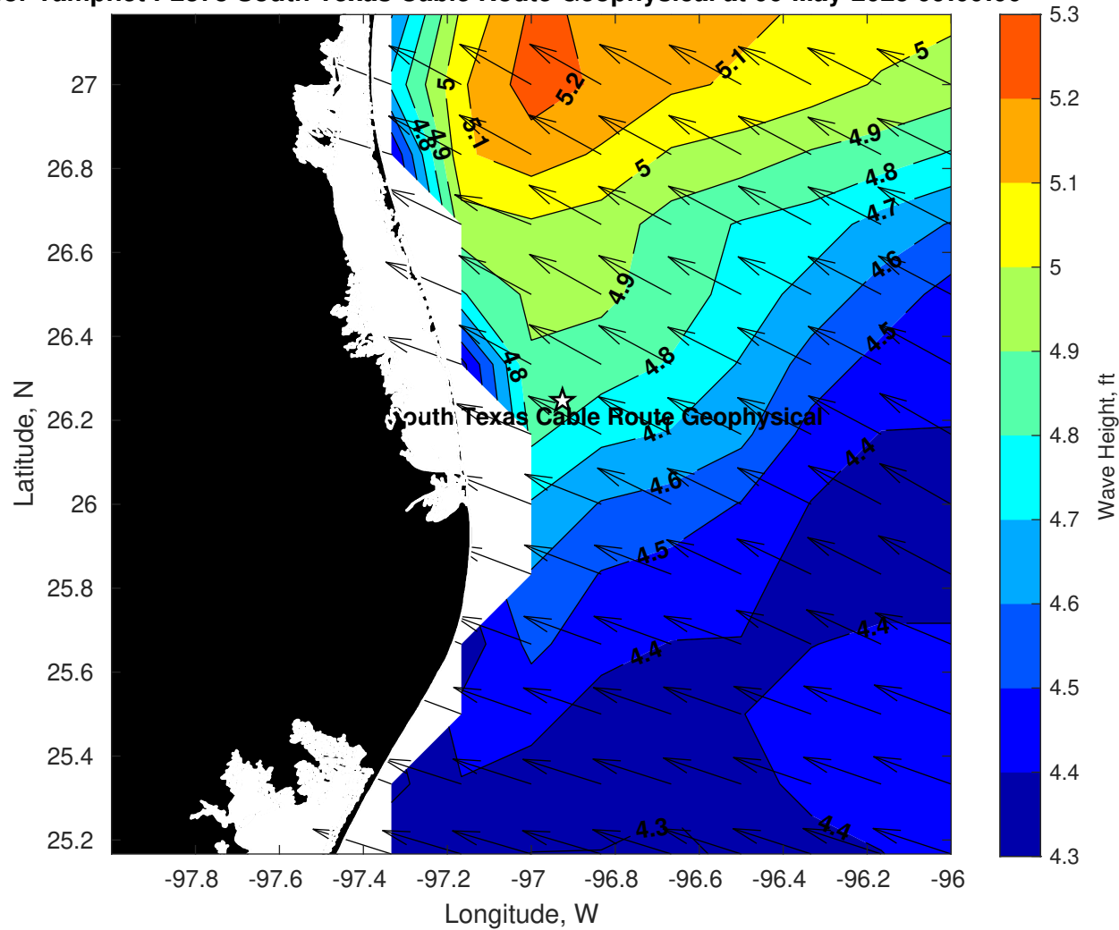
Wave Height (ft) for Tampnet P2378 South Texas Cable Route Geophysical at 06-May-2025 09:00:00
