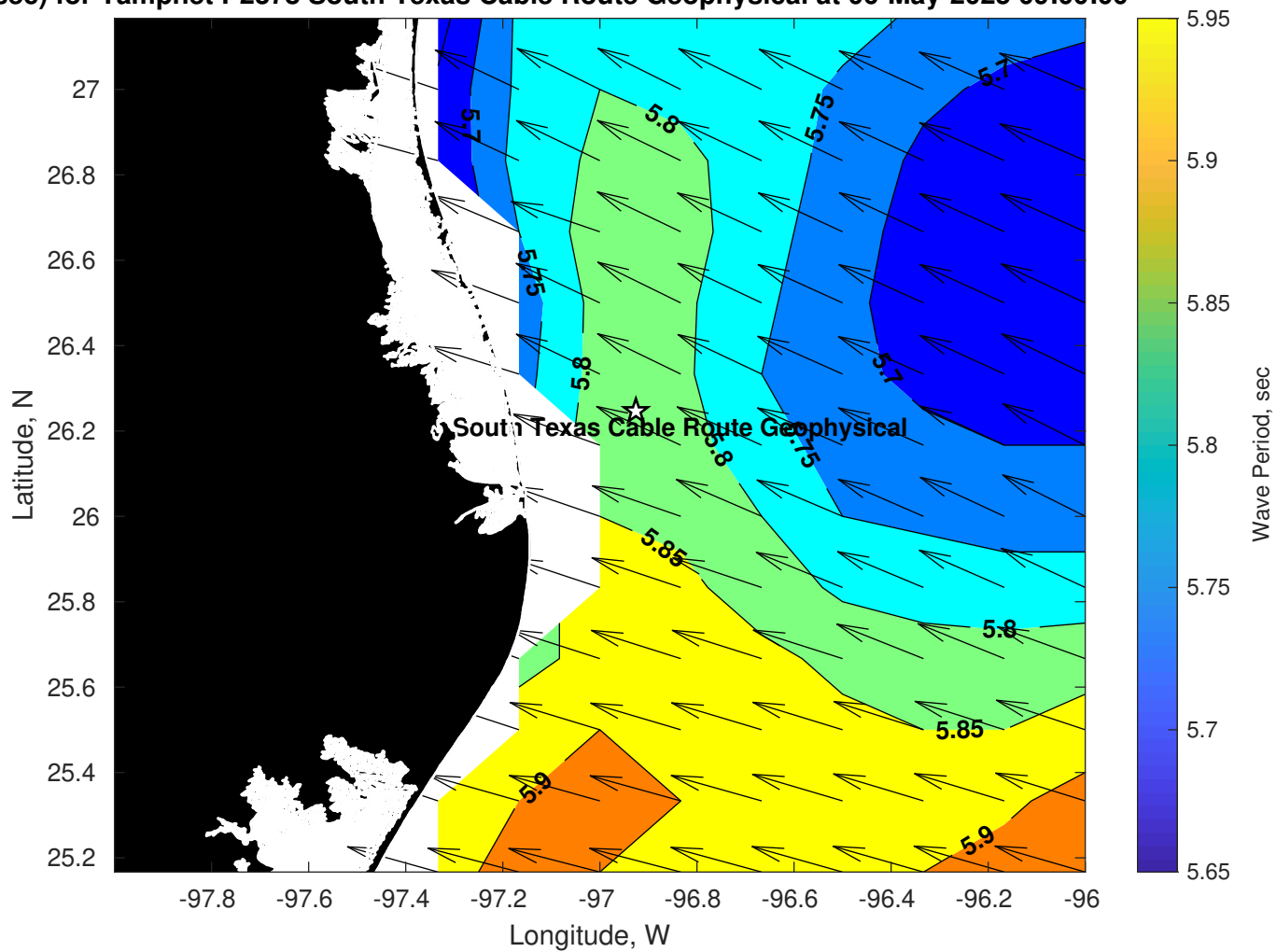
Period (sec) for Tampnet P2378 South Texas Cable Route Geophysical at 06-May-2025 09:00:00
