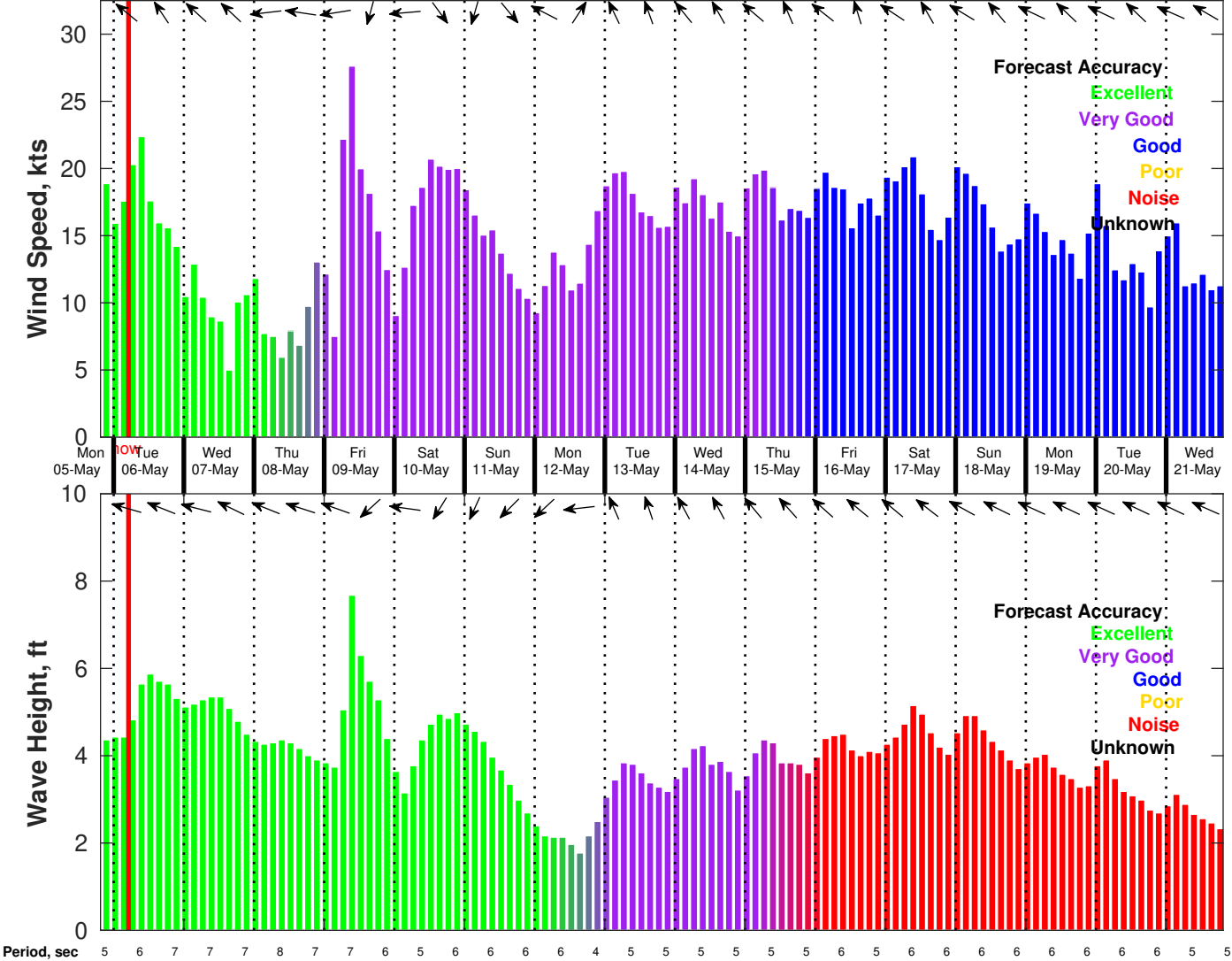
Wind & Wave Forecast for Tampnet P2378 South Texas Cable Route Geophysical from 05-May-2025 20:00:00 to 21-May-2025 20:00:00
