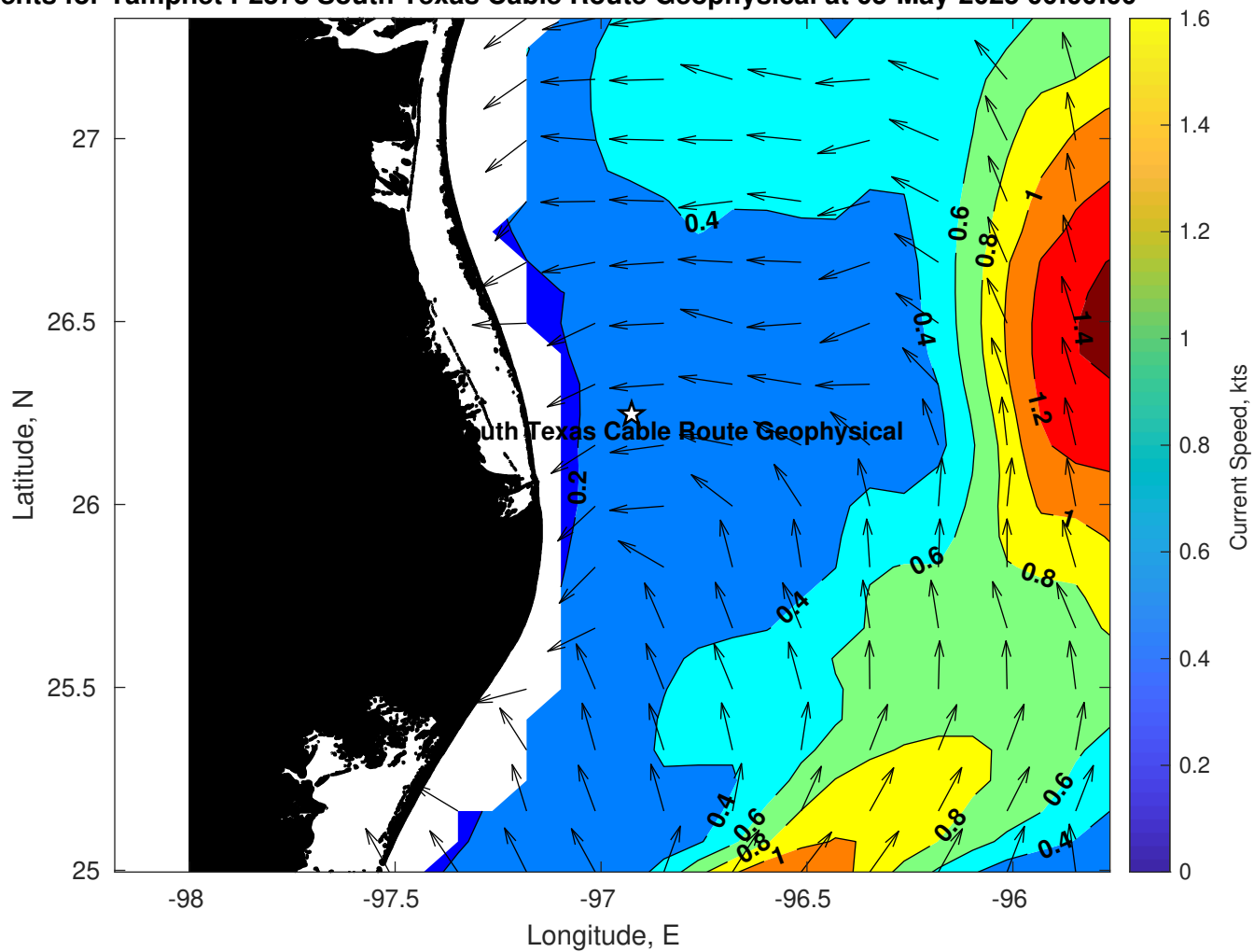
Surface Currents for Tampnet P2378 South Texas Cable Route Geophysical at 05-May-2025 00:00:00
