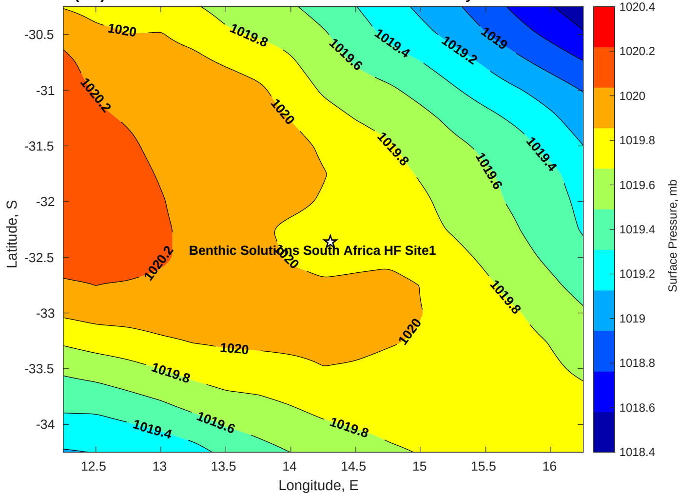
Surface Pressure (mb) for Benthic Solutions South Africa HF Site1 at 08-May-2025 00:00:00
