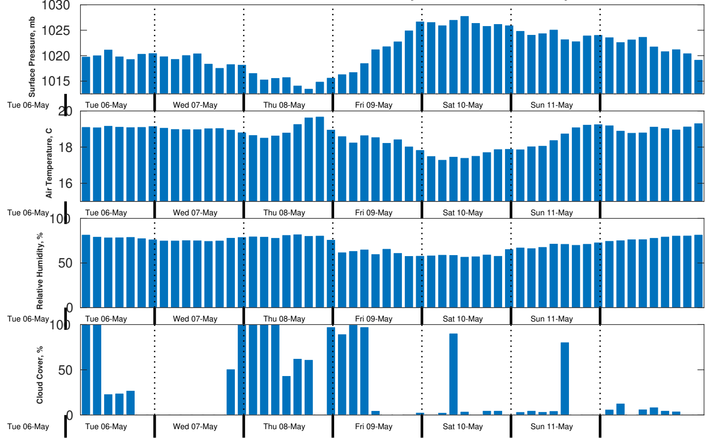
Met Forecast for Benthic Solutions South Africa HF Site1 from 07-May-2025 00:00:00 to 14-May-2025 00:00:00
