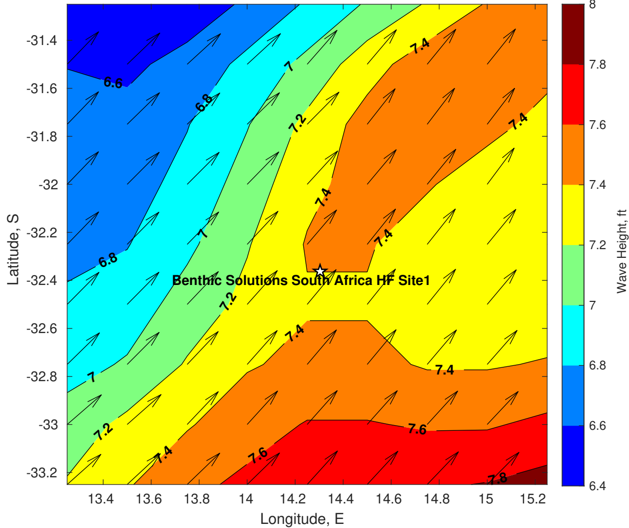
Wave Height (ft) for Benthic Solutions South Africa HF Site1 at 07-May-2025 09:00:00
