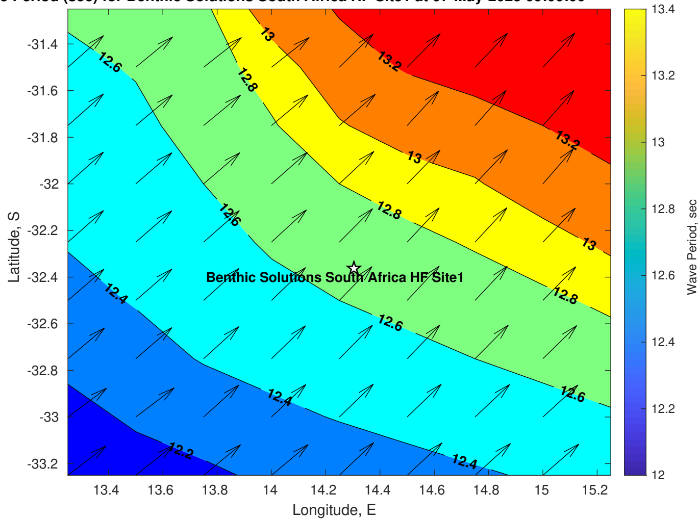
Wave Period (sec) for Benthic Solutions South Africa HF Site1 at 07-May-2025 09:00:00
