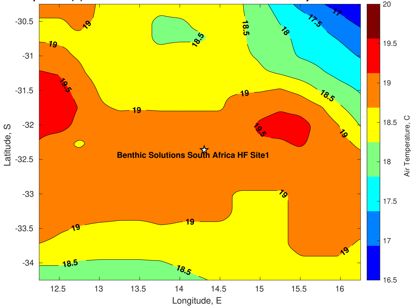
Air Temperature (C) for Benthic Solutions South Africa HF Site1 at 07-May-2025
