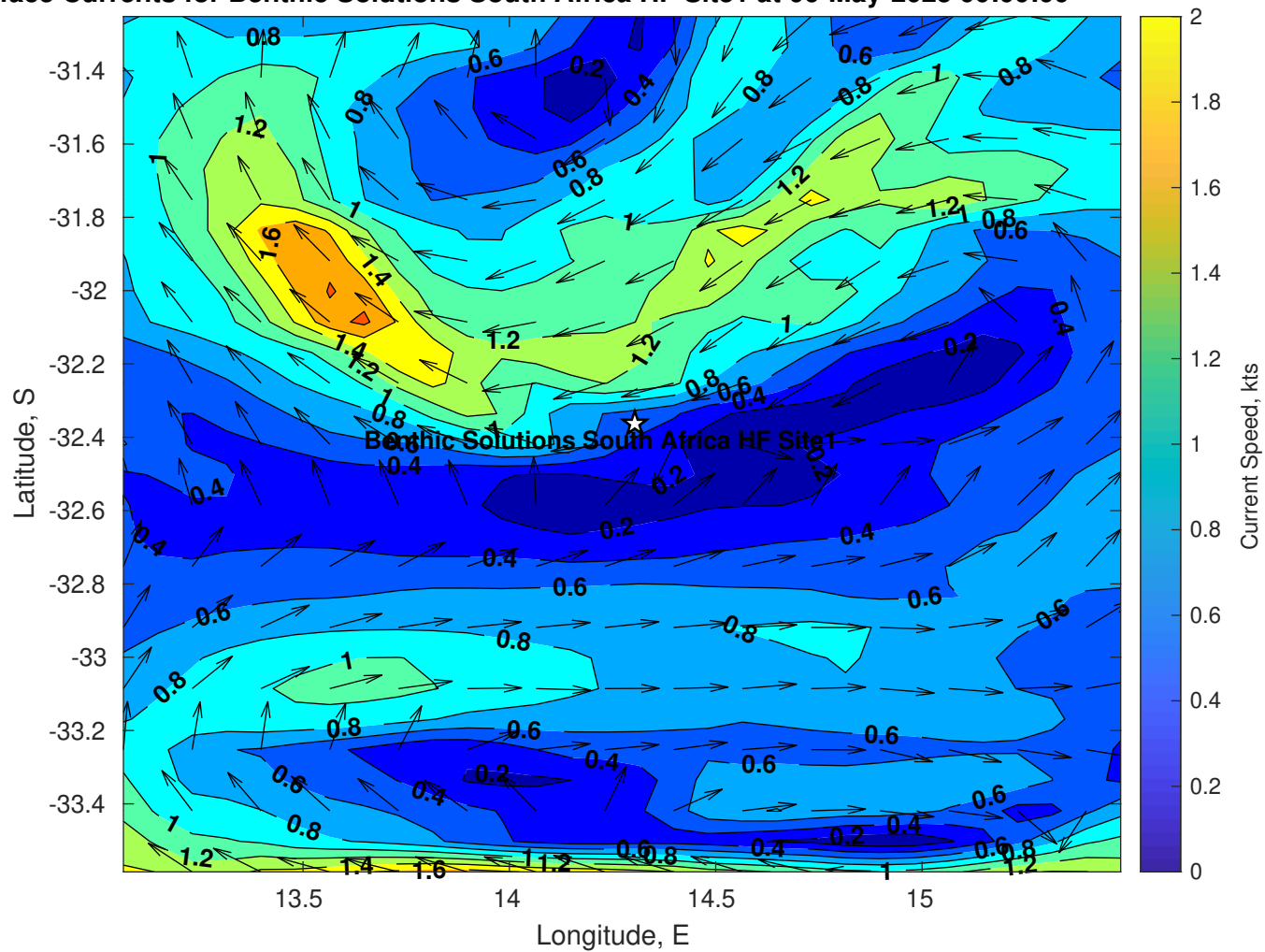
Surface Currents for Benthic Solutions South Africa HF Site1 at 06-May-2025 00:00:00
