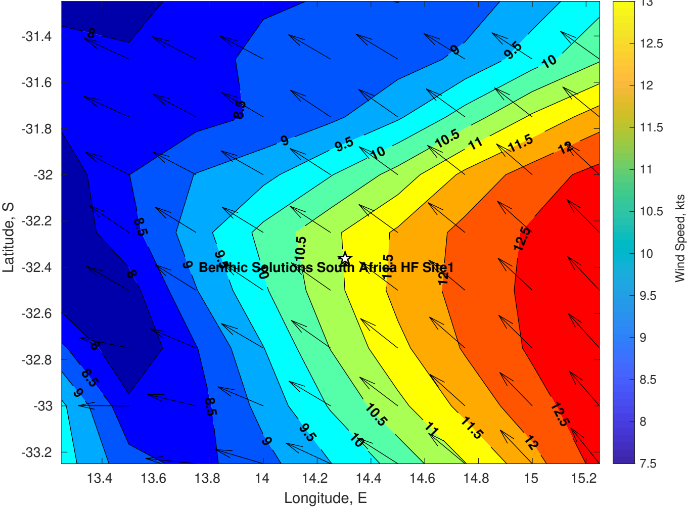
Winds (kts) for Benthic Solutions South Africa HF Site1 at 07-May-2025 09:00:00
