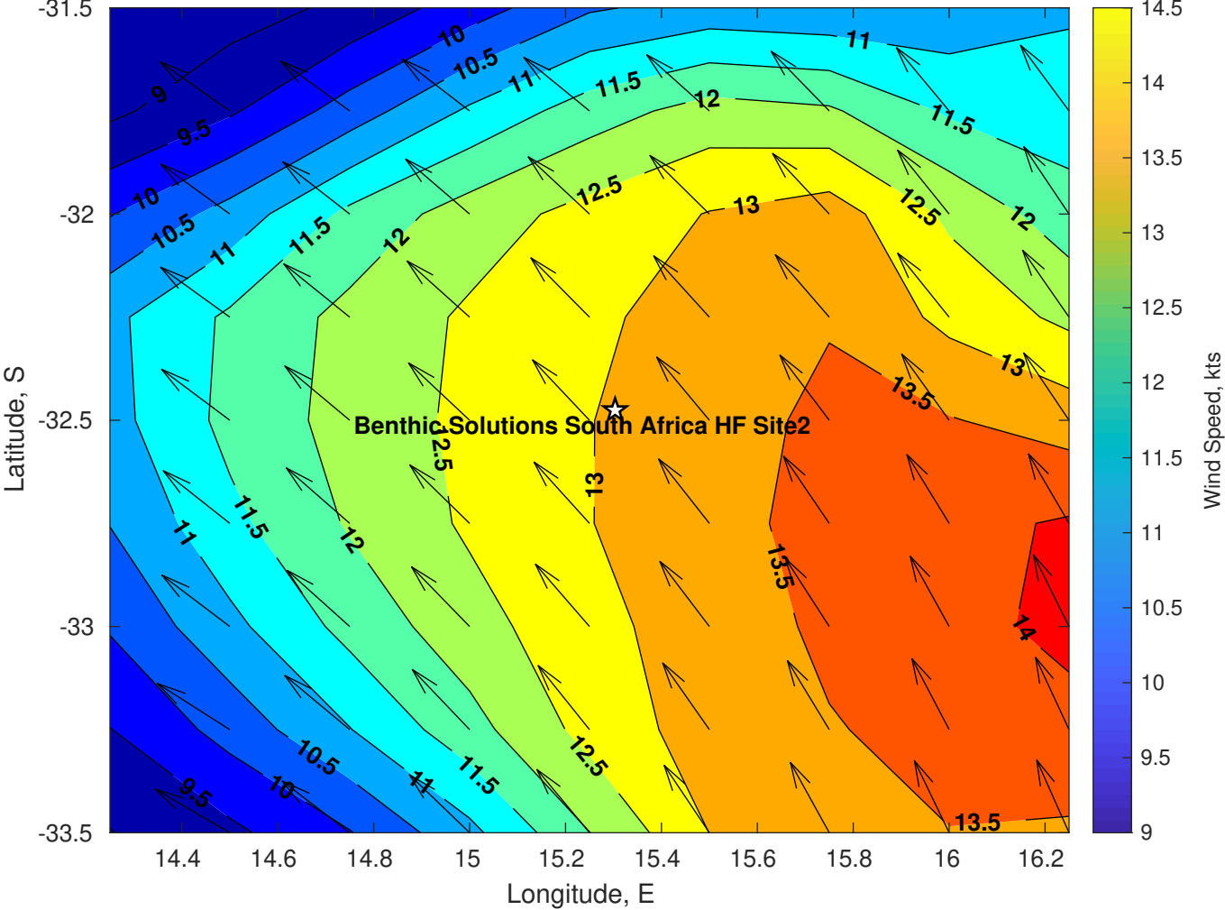
Winds (kts) for Benthic Solutions South Africa HF Site2 at 07-May-2025 09:00:00
