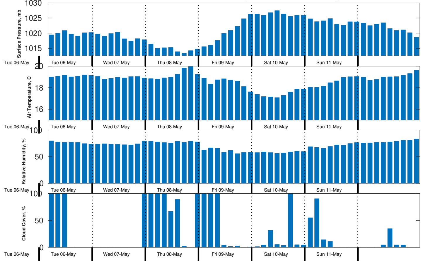
Met Forecast for Benthic Solutions South Africa HF Site2 from 07-May-2025 00:00:00 to 14-May-2025 00:00:00
