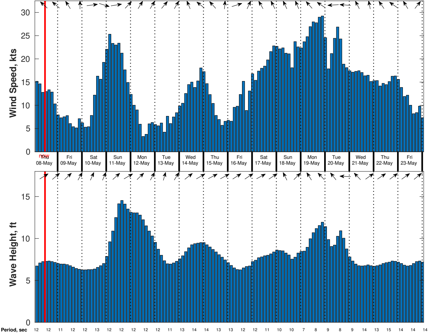
Wind & Wave Forecast for Benthic Solutions South Africa HF Site2 from 07-May-2025 02:00:00 to 23-May-2025 02:00:00
