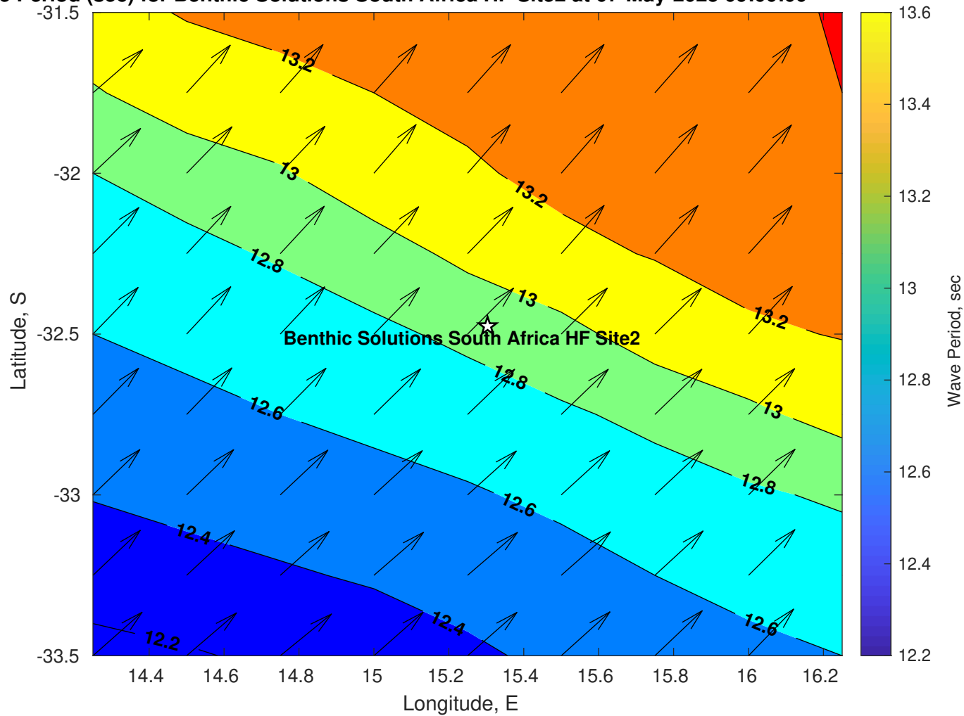
Wave Period (sec) for Benthic Solutions South Africa HF Site2 at 07-May-2025 09:00:00
