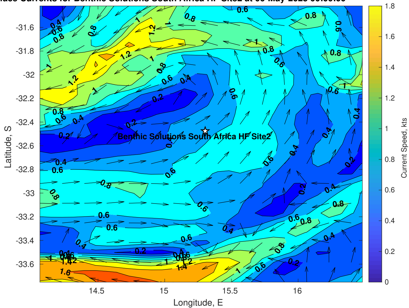
Surface Currents for Benthic Solutions South Africa HF Site2 at 06-May-2025 00:00:00
