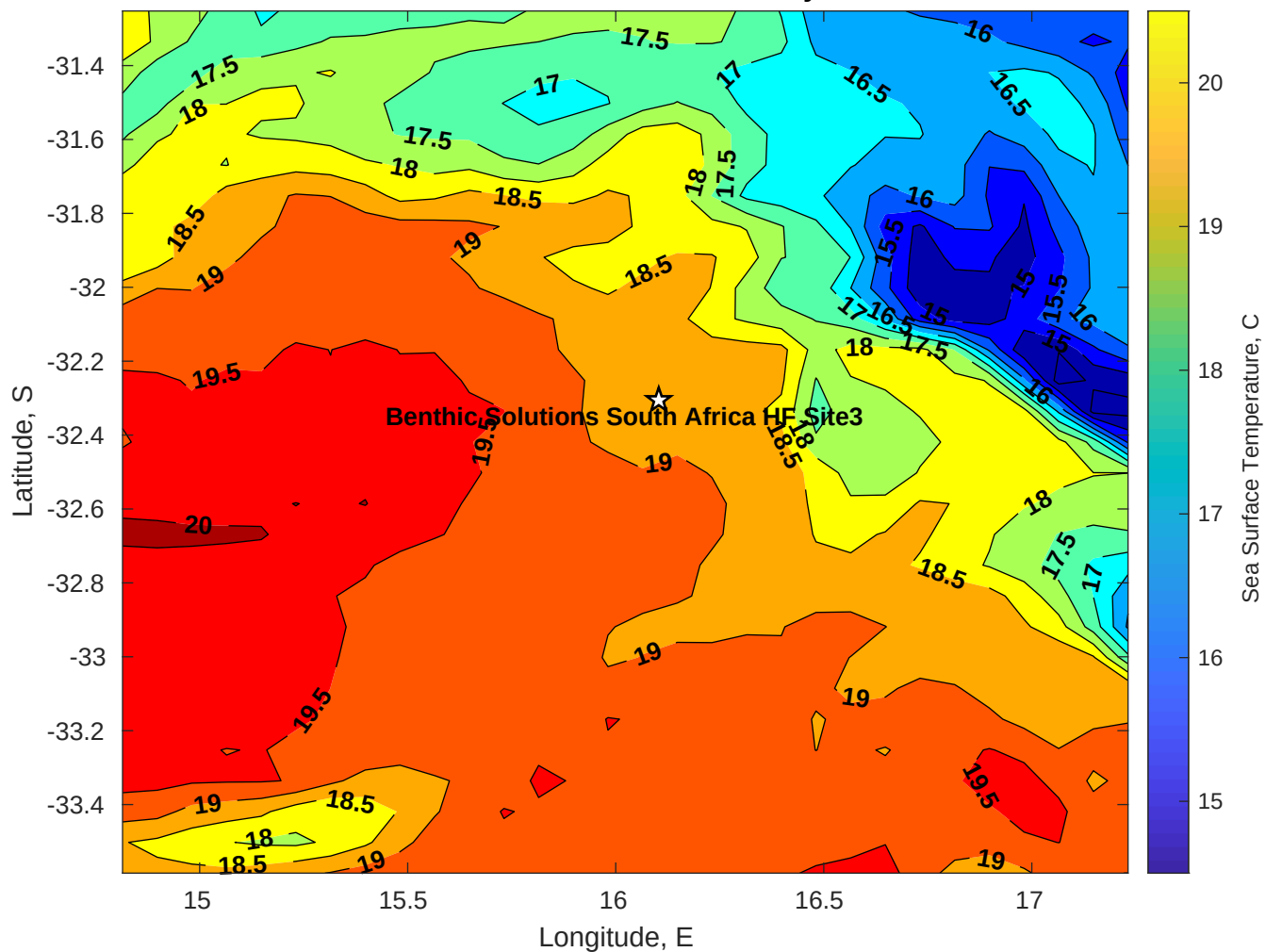
SST for Benthic Solutions South Africa HF Site3 at 06-May-2025 00:00:00
