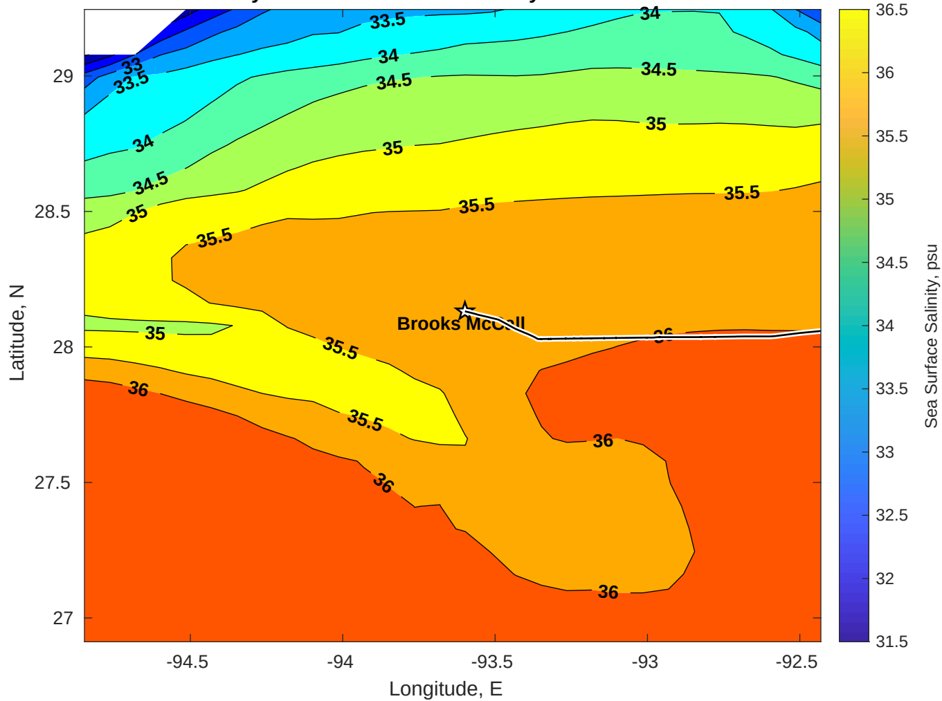
Surface Salinity for Brooks McCall at 06-May-2025 00:00:00
