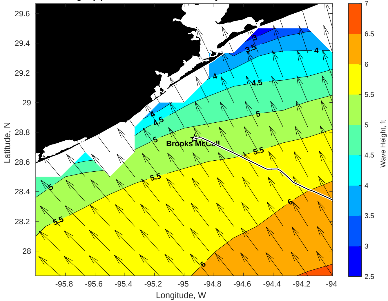
Wave Height (ft) for Brooks McCall at 07-May-2025 09:00:00
