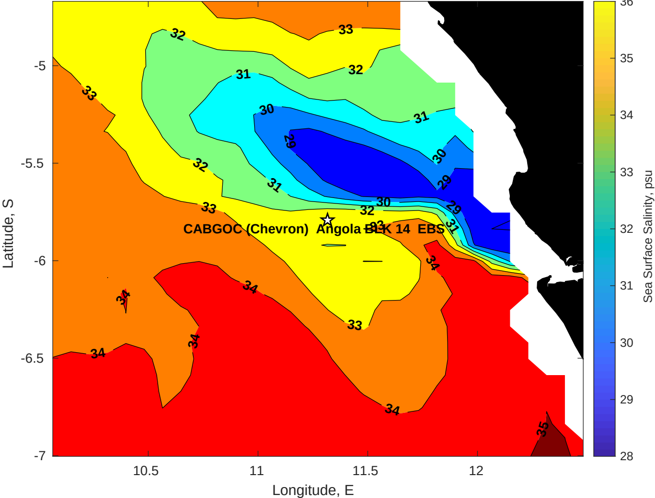
Surface Salinity for CABGOC (Chevron) Angola BLK 14 EBS at 06-May-2025 00:00:00
