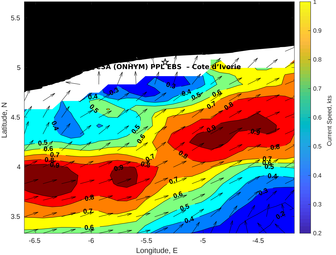
Surface Currents for CSA (ONHYM) PPL EBS - Cote d'Ivoire at 06-May-2025 00:00:00
