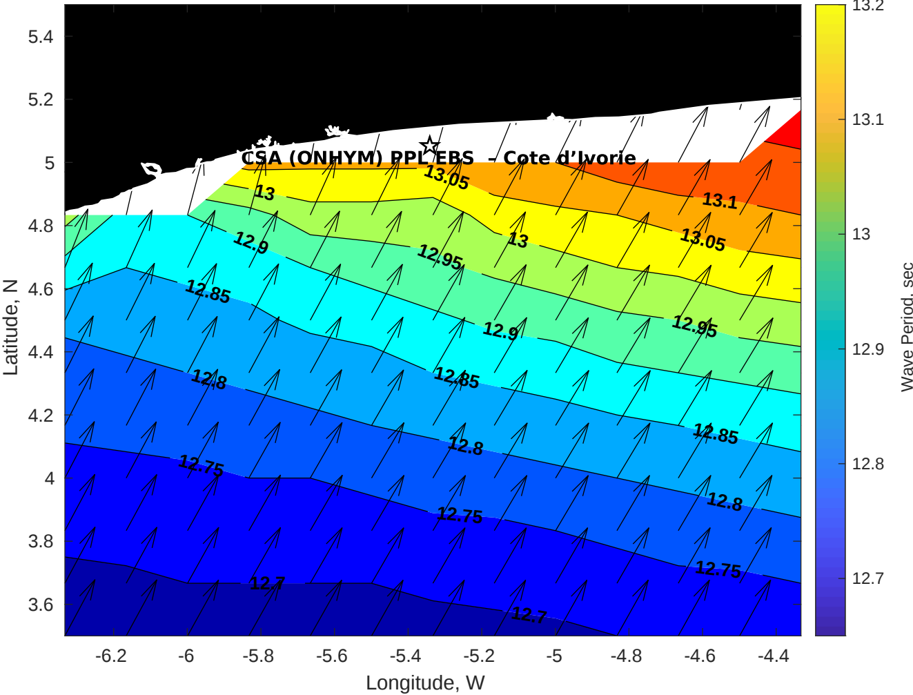
Wave Period (sec) for CSA (ONHYM) PPL EBS - Cote d'Ivoire at 07-May-2025 09:00:00
