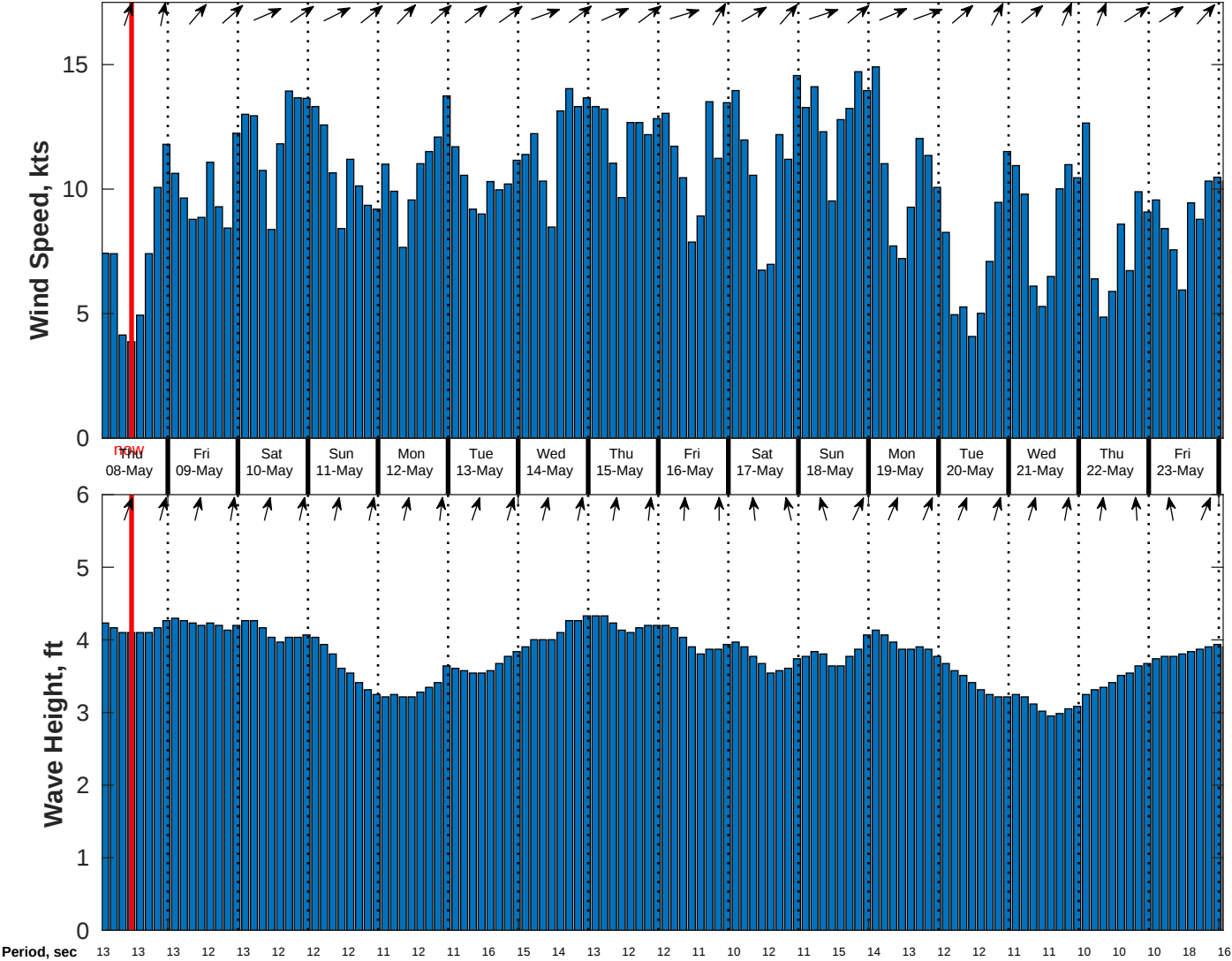
Wind & Wave Forecast for CSA (ONHYM) PPL EBS - Cote d'Ivoire from 07-May-2025 01:00:00 to 23-May-2025 01:00:00
