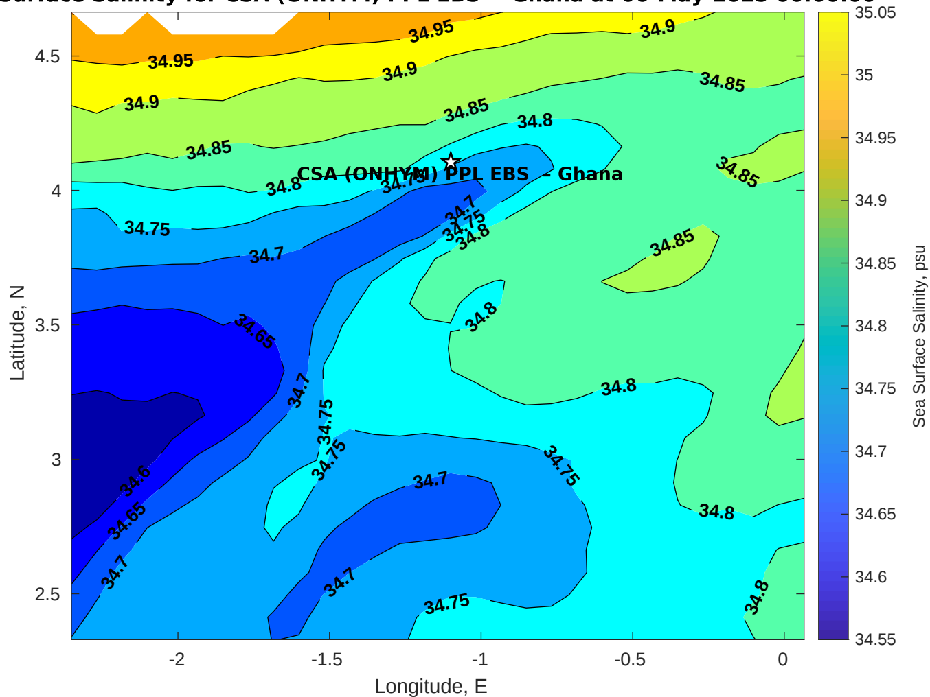
Surface Salinity for CSA (ONHYM) PPL EBS - Ghana at 06-May-2025 00:00:00
