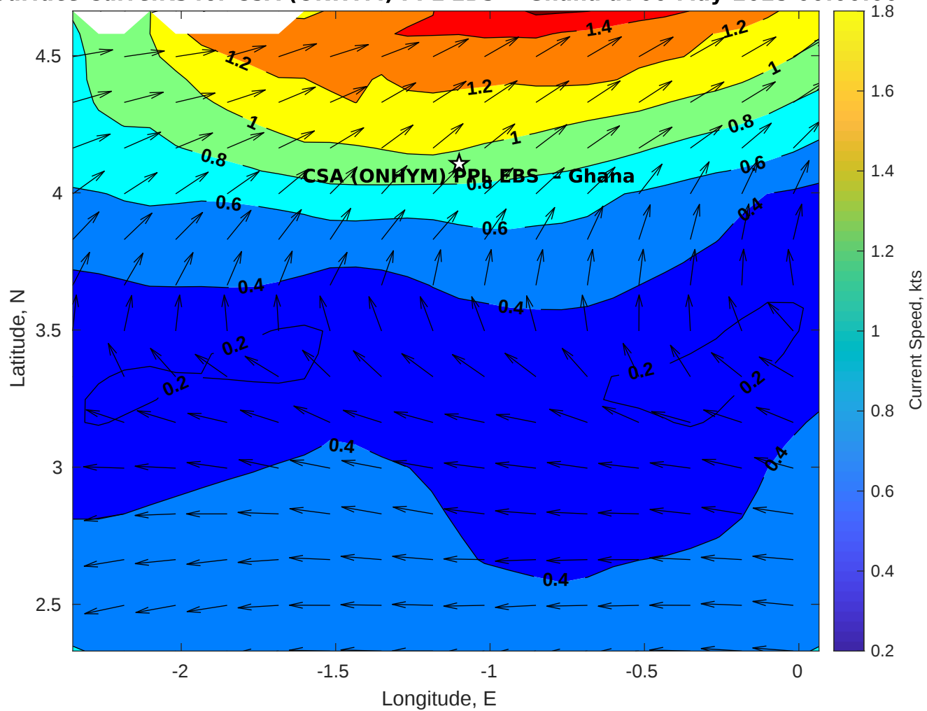
Surface Currents for CSA (ONHYM) PPL EBS - Ghana at 06-May-2025 00:00:00
