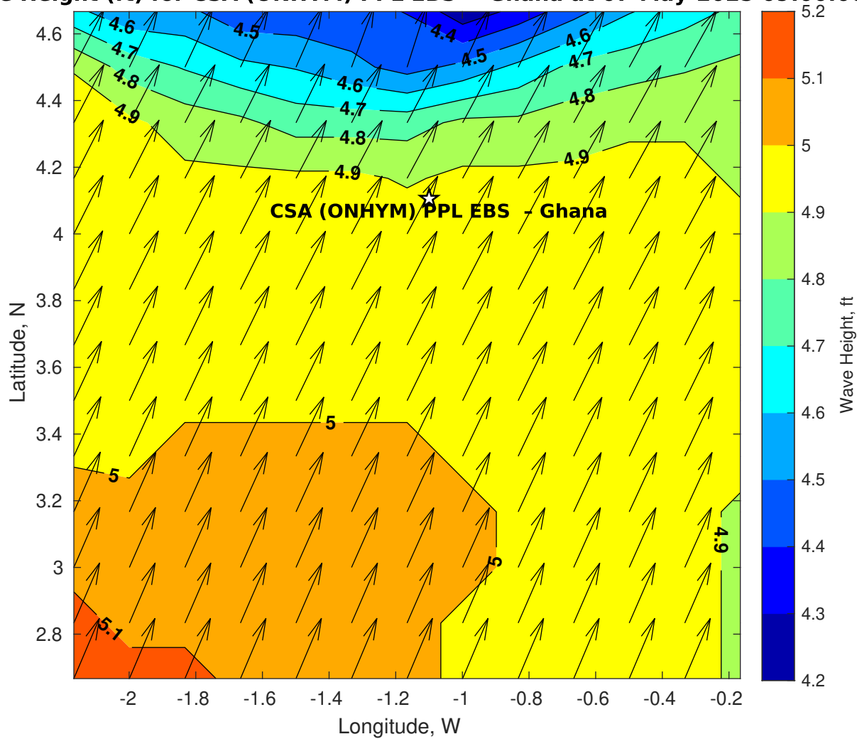
Wave Height (ft) for CSA (ONHYM) PPL EBS - Ghana at 07-May-2025 09:00:00
