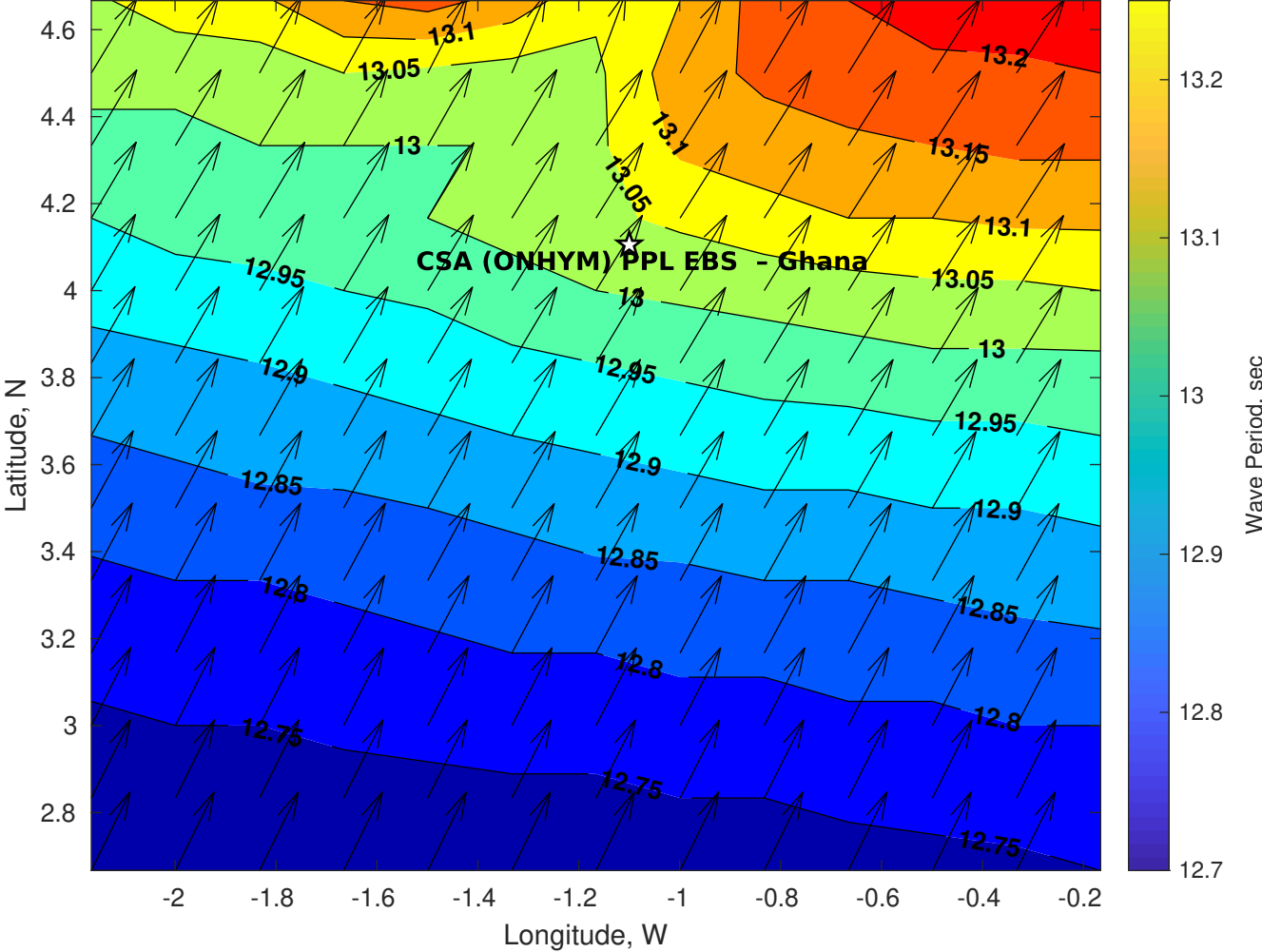
Wave Period (sec) for CSA (ONHYM) PPL EBS - Ghana at 07-May-2025 09:00:00
