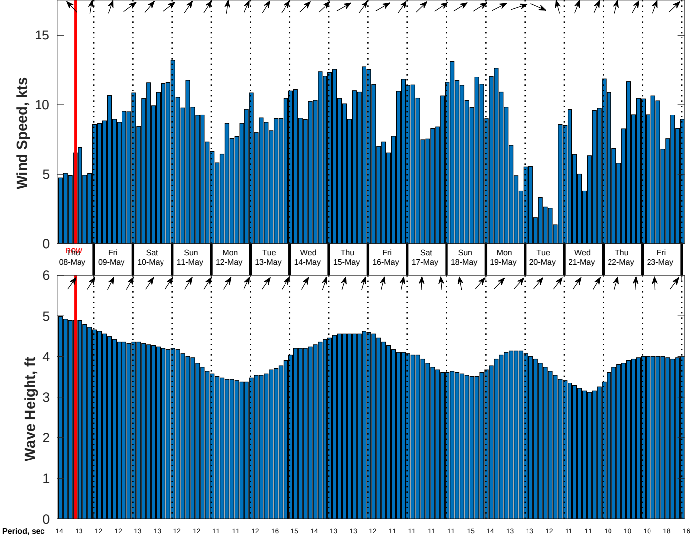
Wind & Wave Forecast for CSA (ONHYM) PPL EBS - Ghana from 07-May-2025 02:00:00 to 23-May-2025 02:00:00
