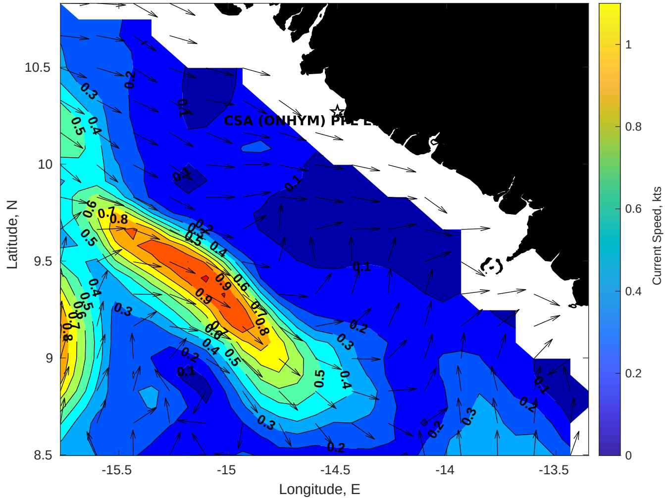
Surface Currents for CSA (ONHYM) PPL EBS - Guinea at 06-May-2025 00:00:00
