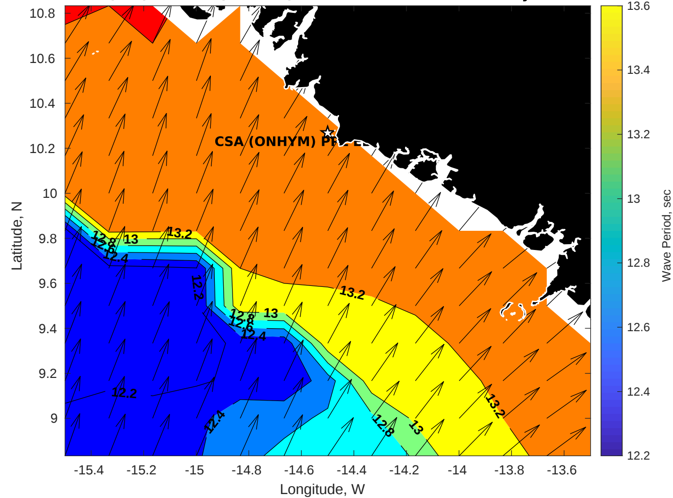
Wave Period (sec) for CSA (ONHYM) PPL EBS - Guinea at 07-May-2025 09:00:00
