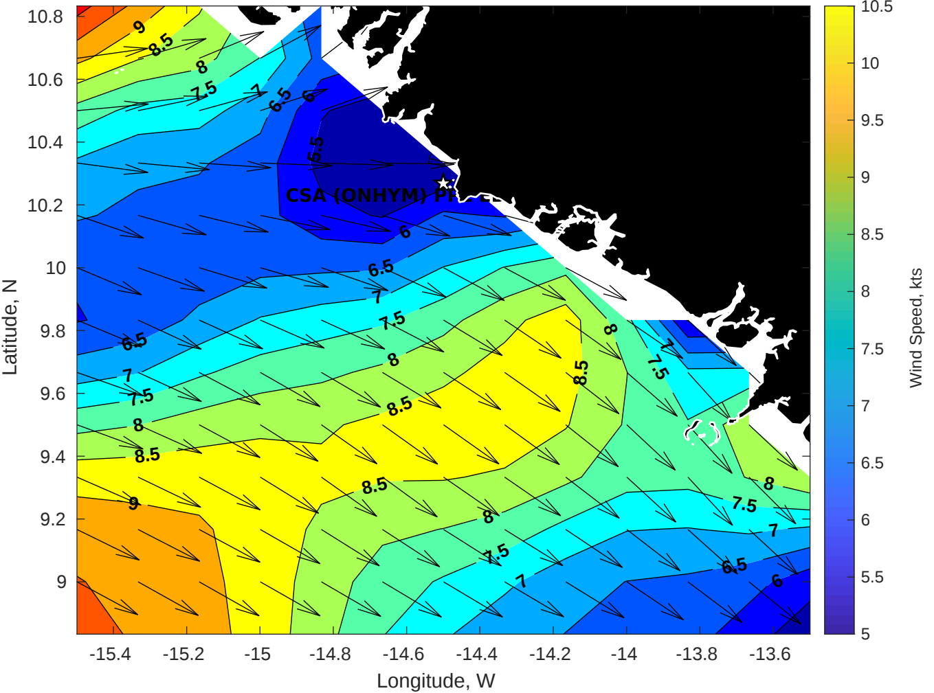
Winds (kts) for CSA (ONHYM) PPL EBS - Guinea at 07-May-2025 09:00:00
