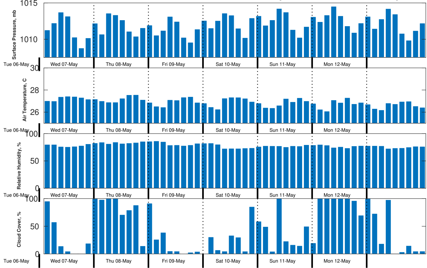
Met Forecast for CSA (ONHYM) PPL EBS - Guinea from 07-May-2025 00:00:00 to 14-May-2025 00:00:00
