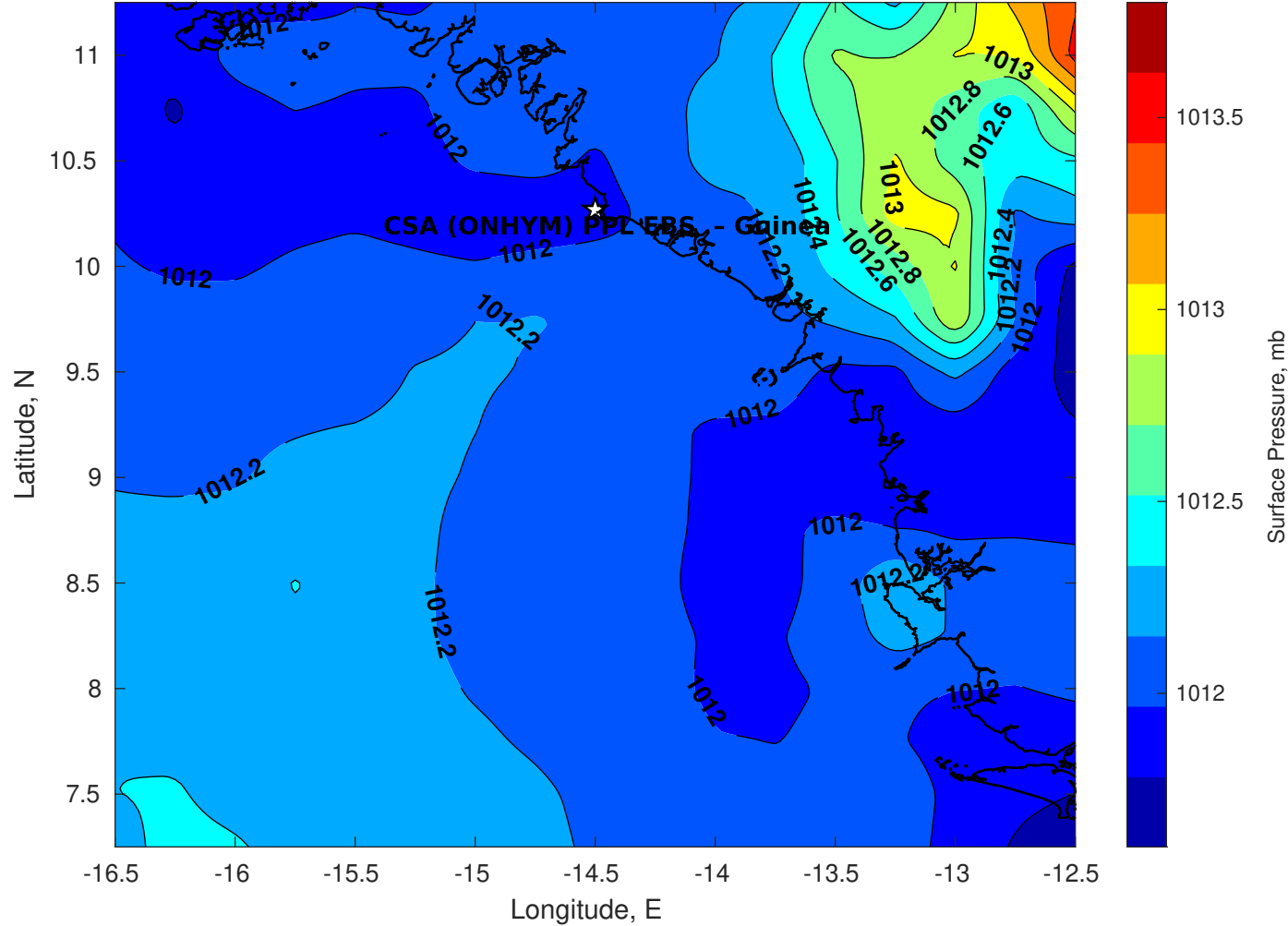
Surface Pressure (mb) for CSA (ONHYM) PPL EBS - Guinea at 09-May-2025 00:00:00
