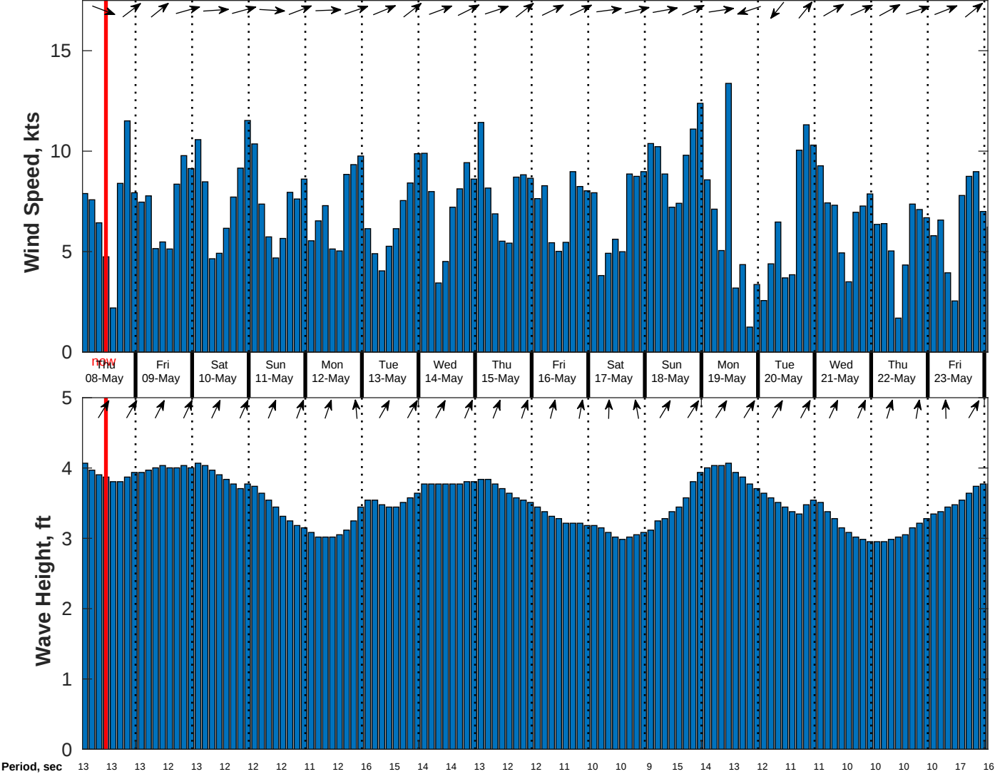
Wind & Wave Forecast for CSA (ONHYM) PPL EBS - Liberia from 07-May-2025 01:00:00 to 23-May-2025 01:00:00
