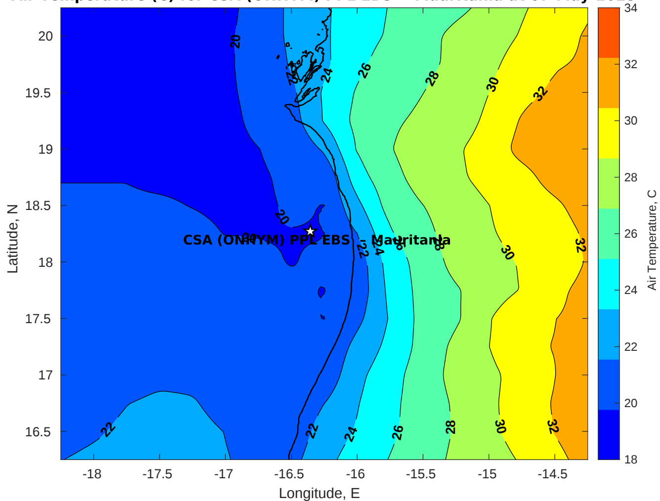
Air Temperature (C) for CSA (ONHYM) PPL EBS - Mauritania at 07-May-2025
