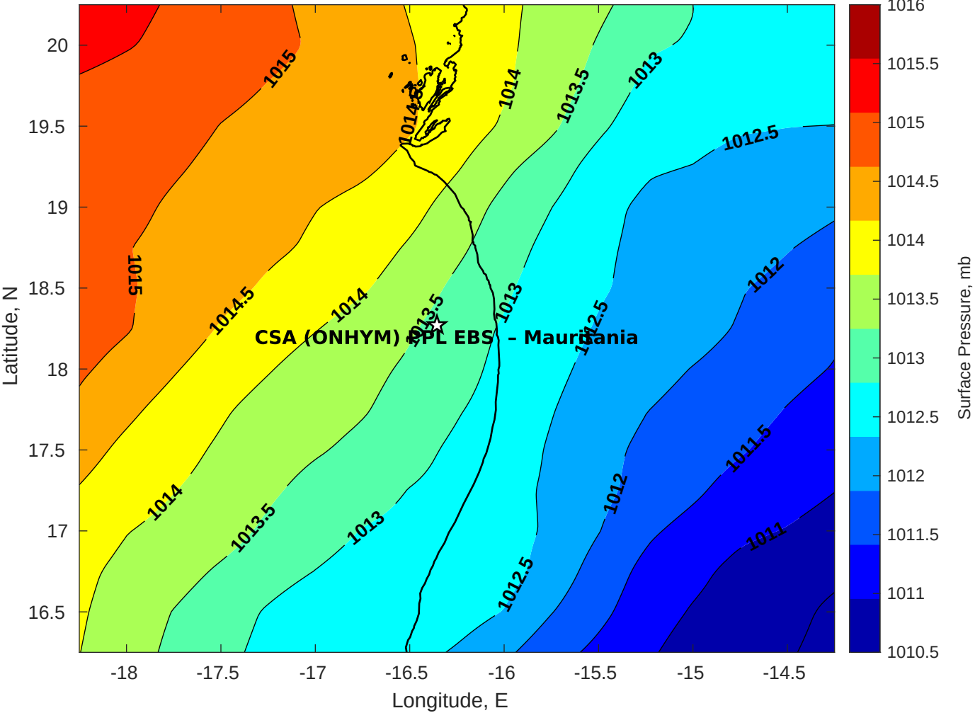
Surface Pressure (mb) for CSA (ONHYM) PPL EBS - Mauritania at 07-May-2025 00:00:00
