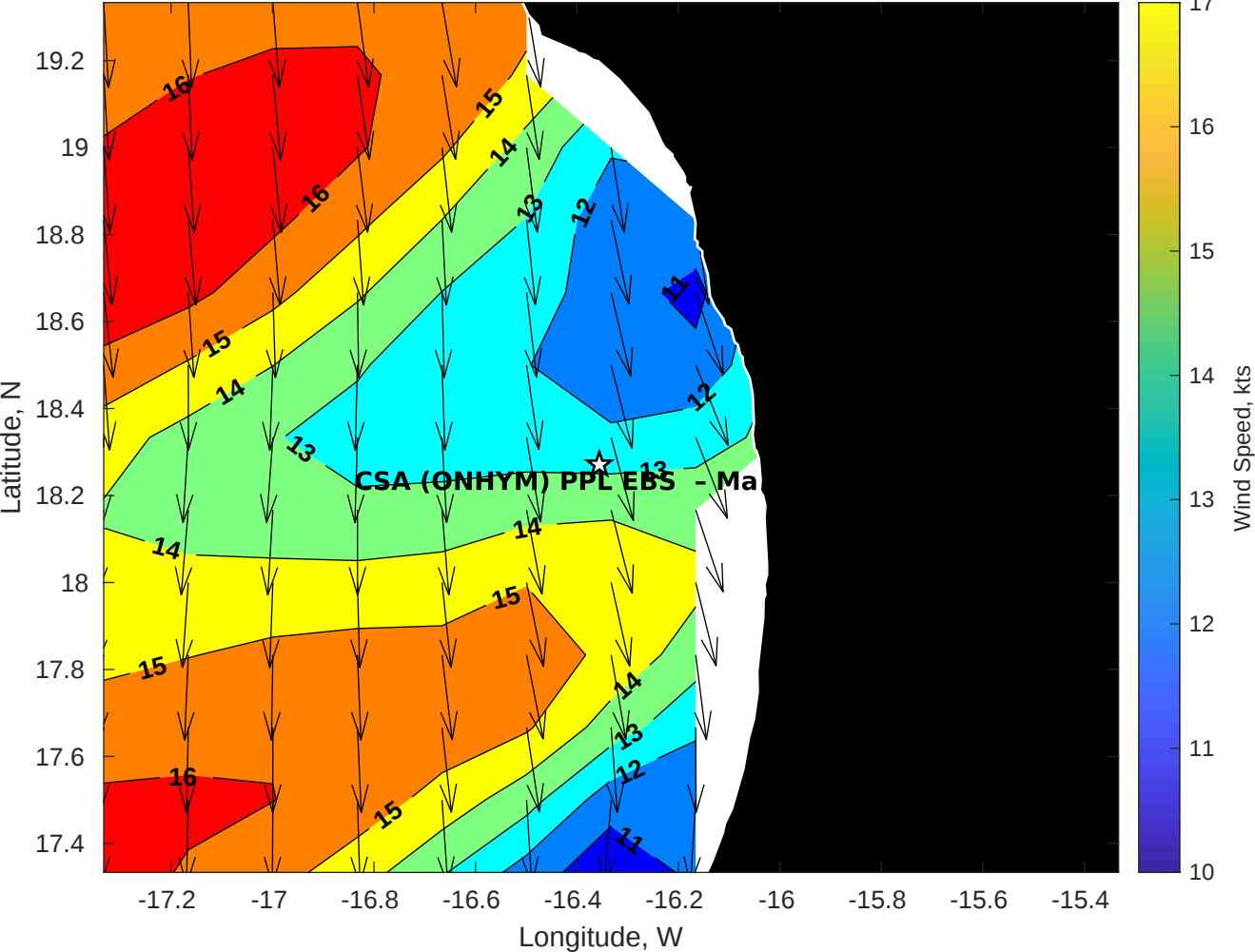
Winds (kts) for CSA (ONHYM) PPL EBS - Mauritania at 07-May-2025 09:00:00
