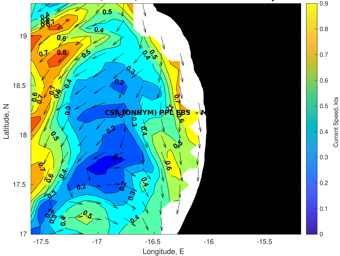
Surface Currents for CSA (ONHYM) PPL EBS - Mauritania at 06-May-2025 00:00:00
