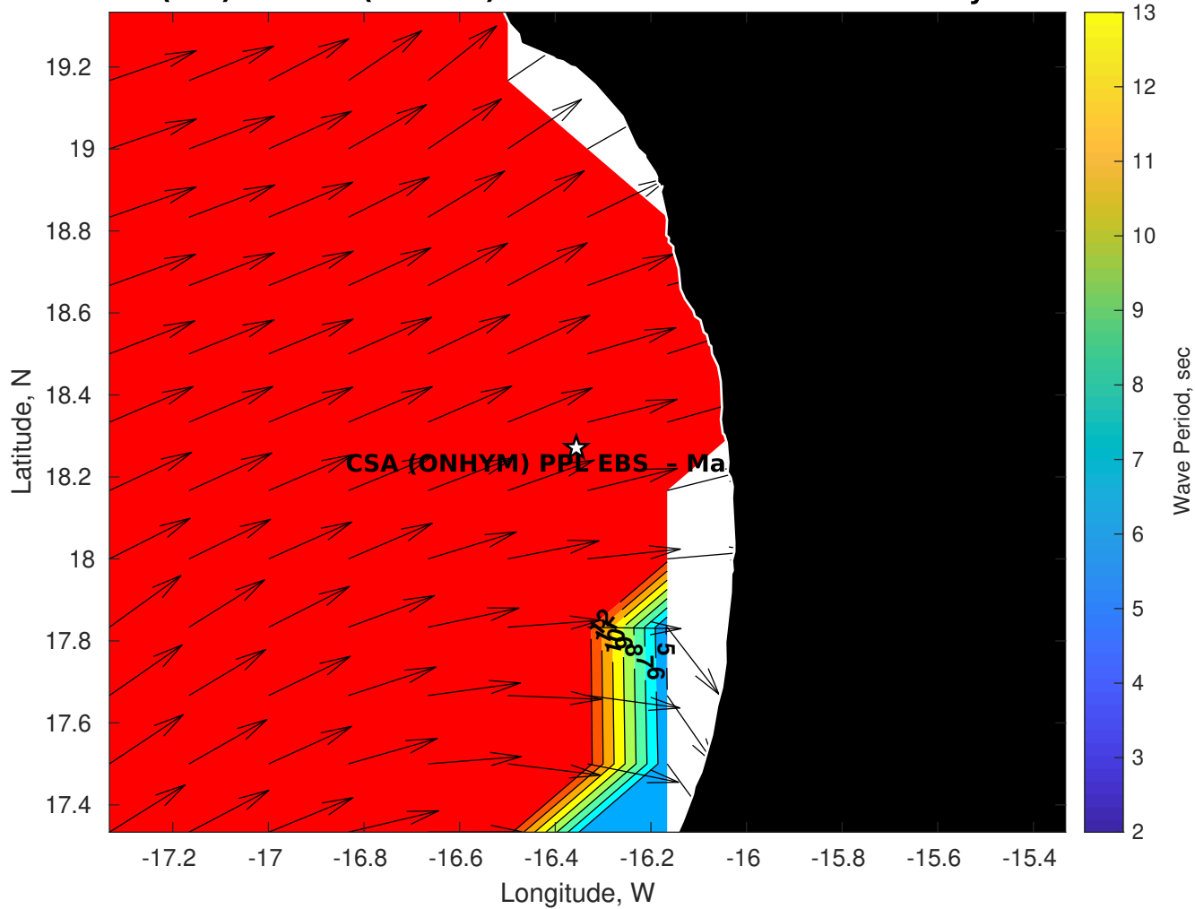
Wave Period (sec) for CSA (ONHYM) PPL EBS - Mauritania at 07-May-2025 09:00:00
