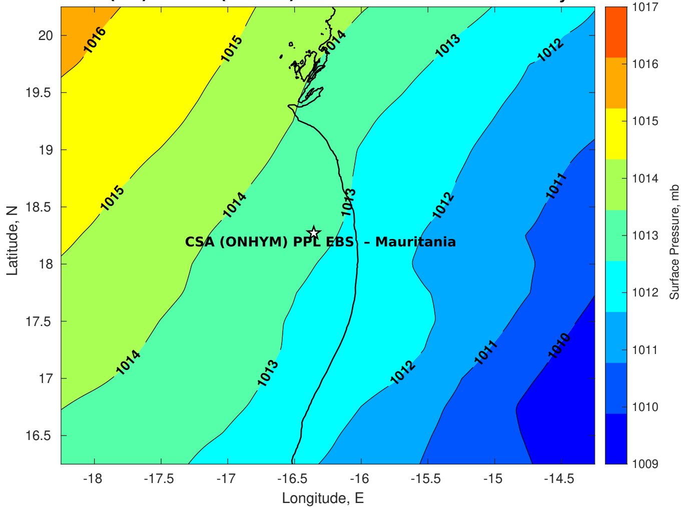
Surface Pressure (mb) for CSA (ONHYM) PPL EBS - Mauritania at 08-May-2025 00:00:00
