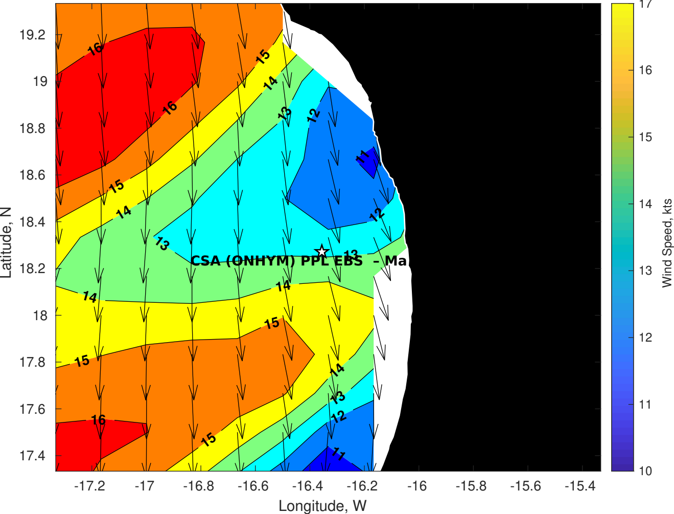
Winds (kts) for CSA (ONHYM) PPL EBS - Mauritania at 07-May-2025 09:00:00
