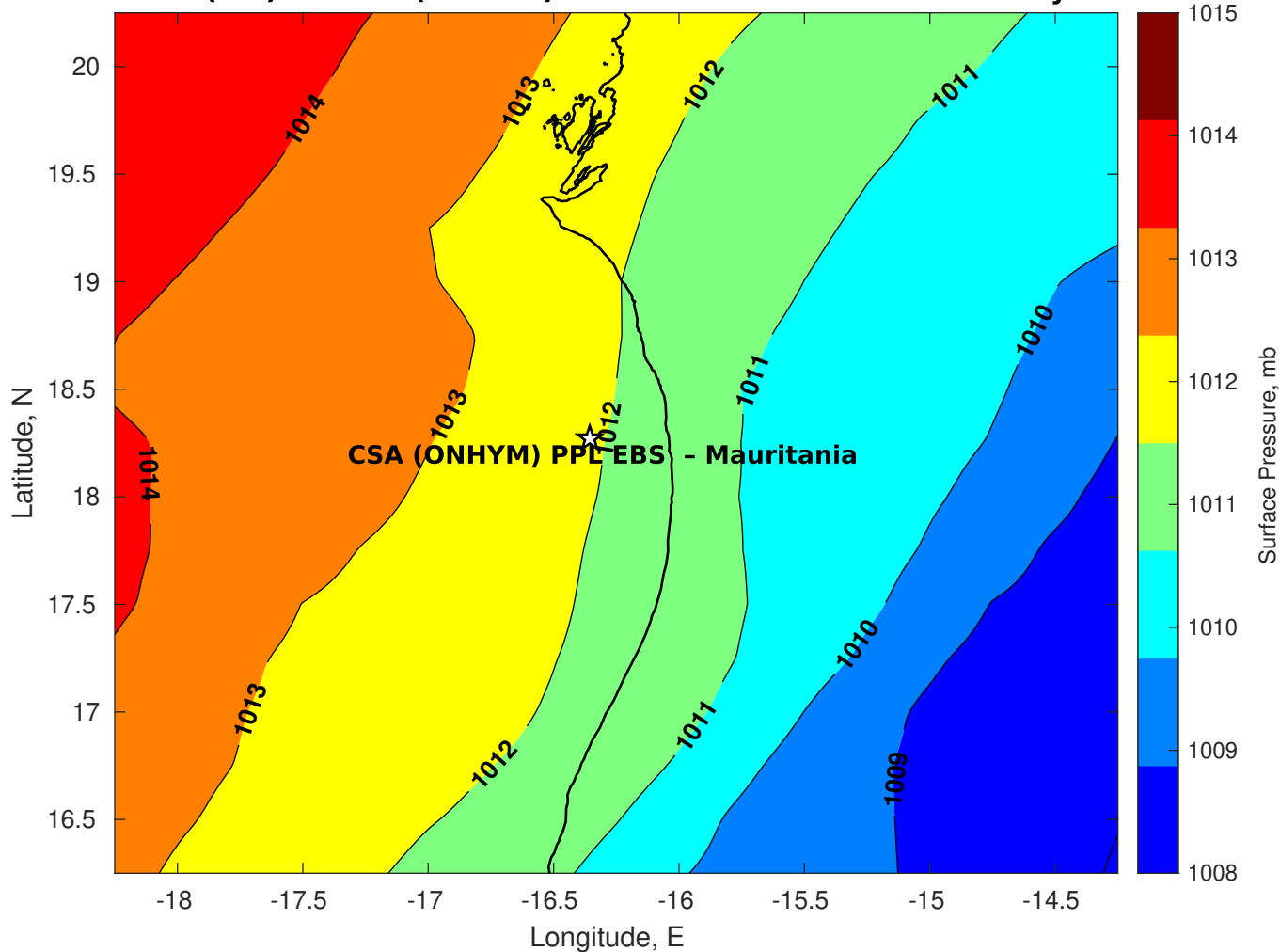
Surface Pressure (mb) for CSA (ONHYM) PPL EBS - Mauritania at 09-May-2025 00:00:00
