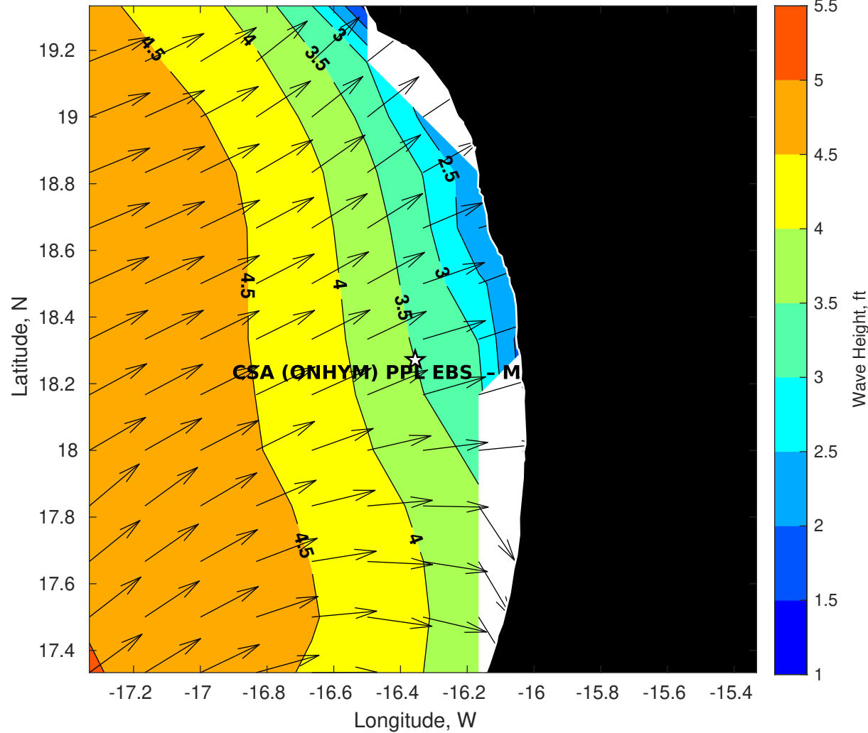
Wave Height (ft) for CSA (ONHYM) PPL EBS - Mauritania at 07-May-2025 09:00:00
