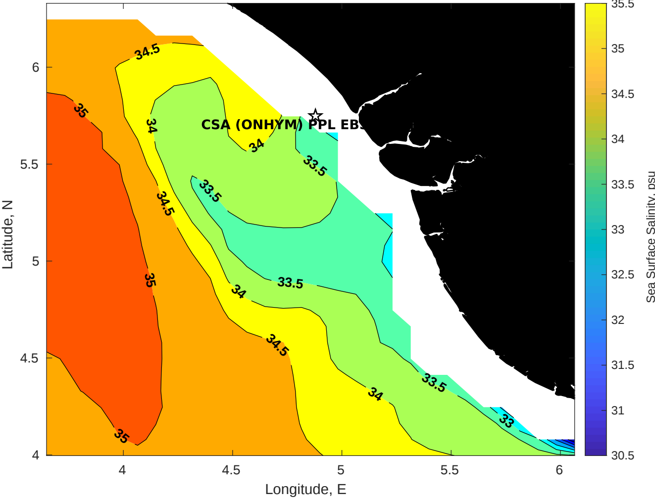
Surface Salinity for CSA (ONHYM) PPL EBS - Nigeria at 06-May-2025 00:00:00
