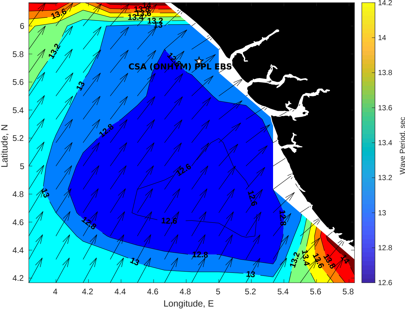
Wave Period (sec) for CSA (ONHYM) PPL EBS - Nigeria at 07-May-2025 09:00:00
