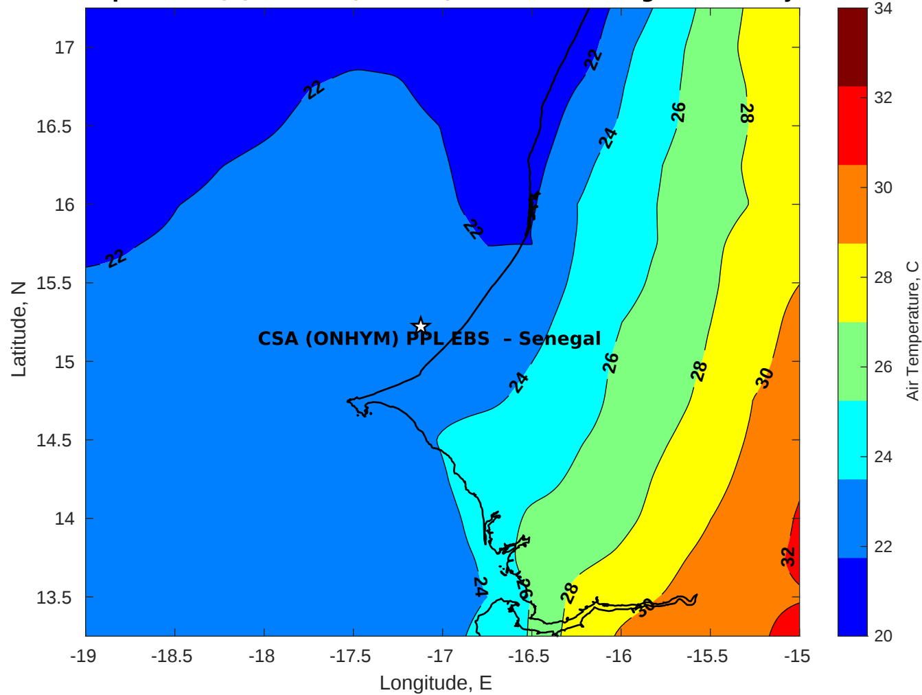
Air Temperature (C) for CSA (ONHYM) PPL EBS - Senegal at 07-May-2025
