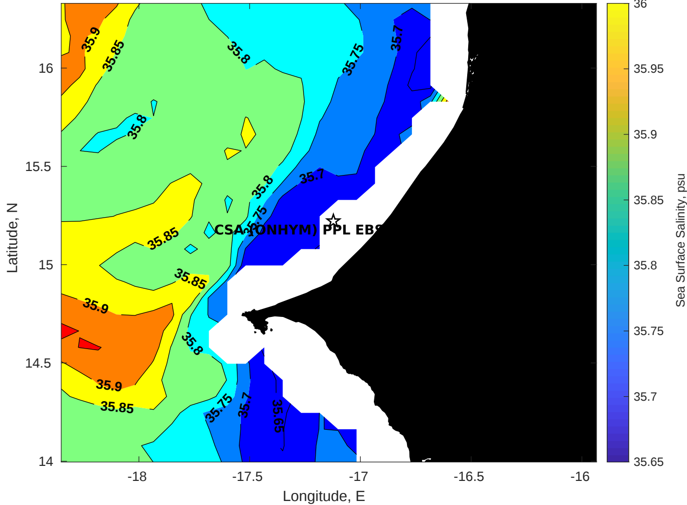
Surface Salinity for CSA (ONHYM) PPL EBS - Senegal at 06-May-2025 00:00:00
