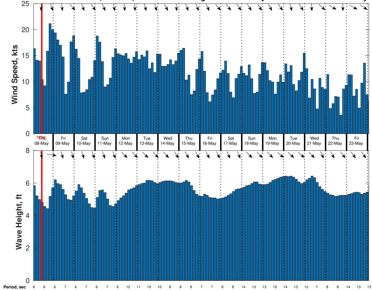
Wind & Wave Forecast for CSA (ONHYM) PPL EBS - Senegal from 07-May-2025 01:00:00 to 23-May-2025 01:00:00
