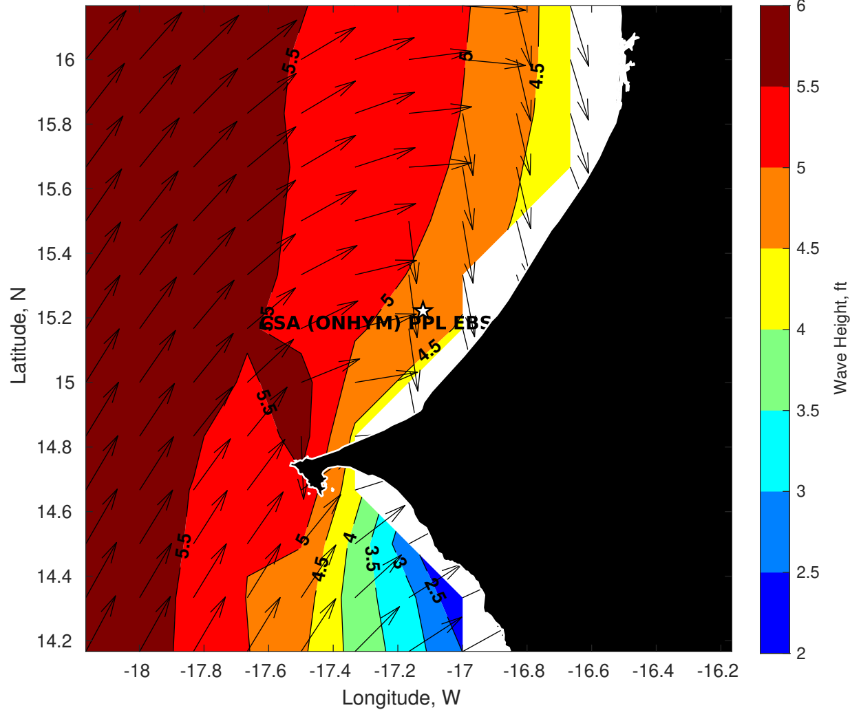
Wave Height (ft) for CSA (ONHYM) PPL EBS - Senegal at 07-May-2025 09:00:00
