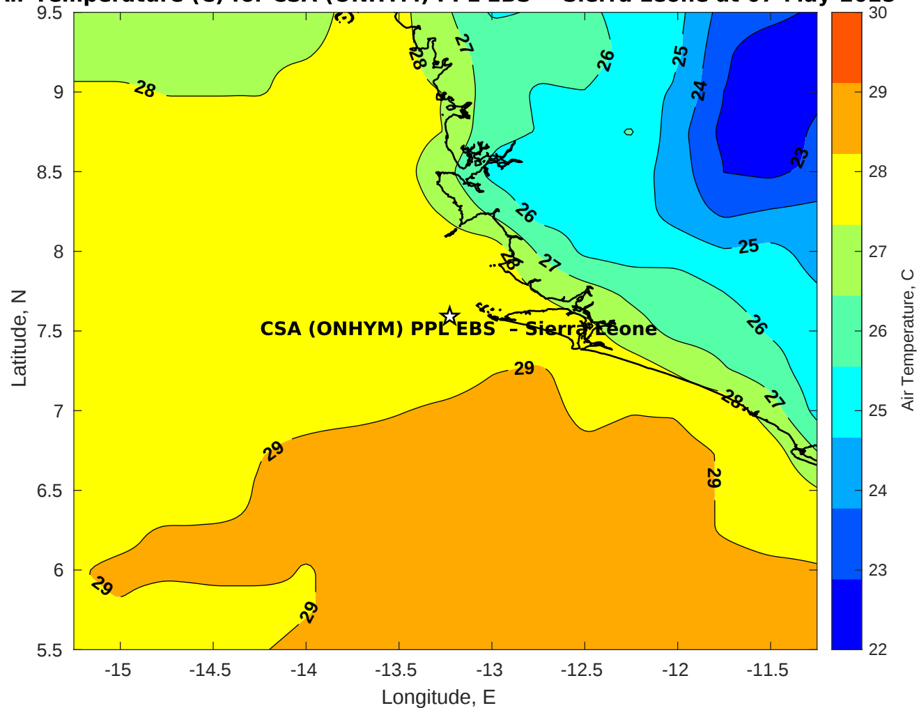
Air Temperature (C) for CSA (ONHYM) PPL EBS - Sierra Leone at 07-May-2025
