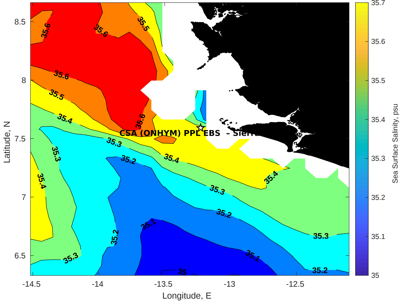
Surface Salinity for CSA (ONHYM) PPL EBS - Sierra Leone at 06-May-2025 00:00:00
