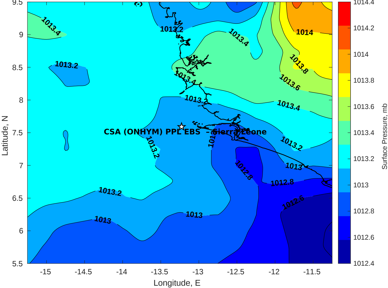
Surface Pressure (mb) for CSA (ONHYM) PPL EBS - Sierra Leone at 07-May-2025 00:00:00
